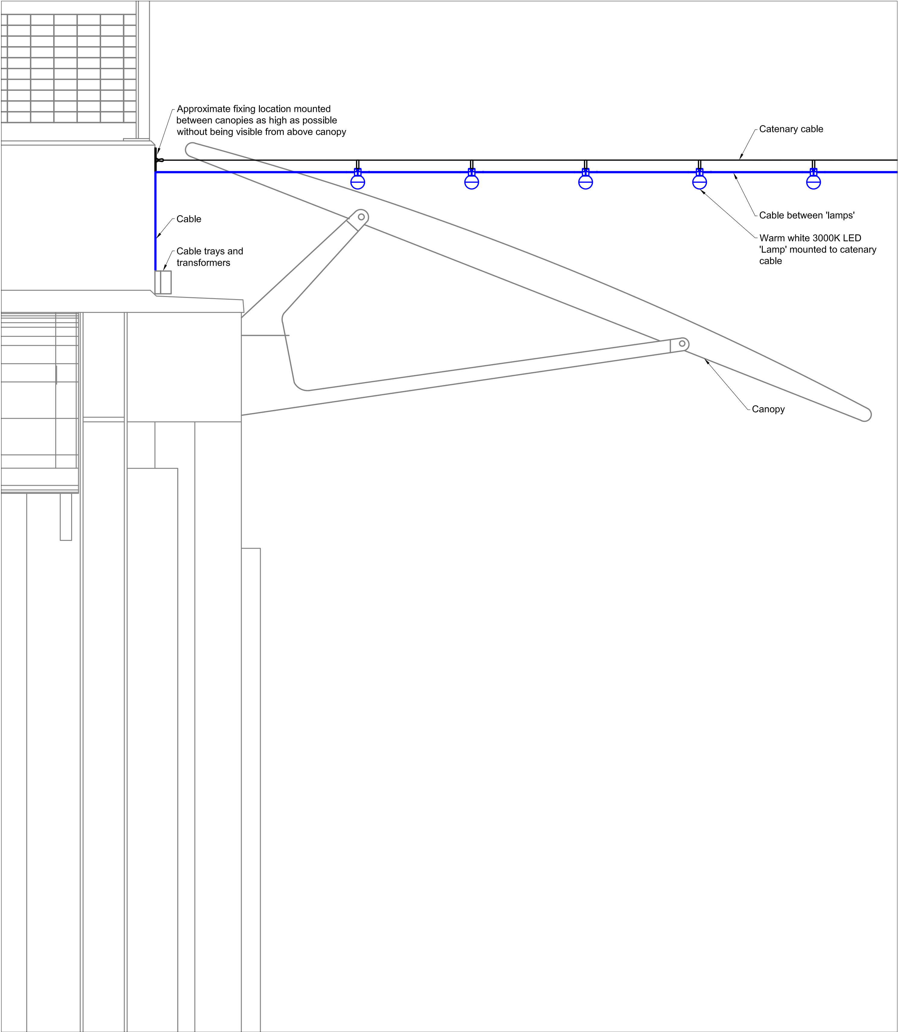
Festoon lighting Section
