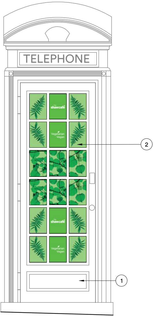
Elevation A1 - Front Box Access As Proposed 1:20
