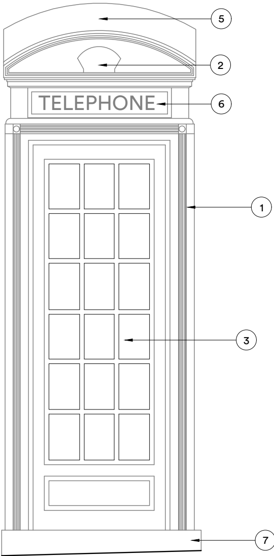
Elevation A2 As Existing 1:20
