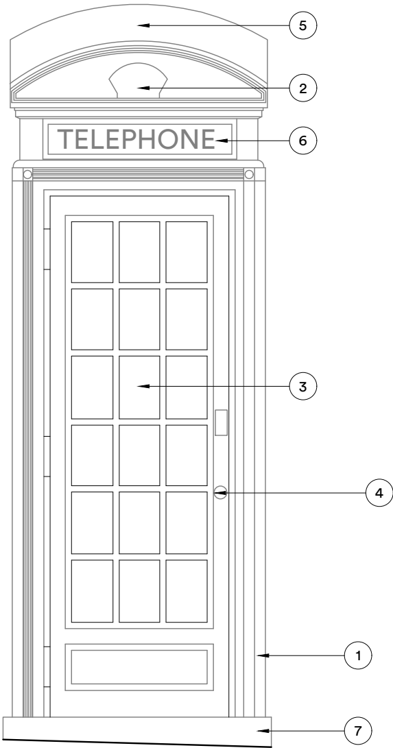
Elevation A1 As Existing 1:20
