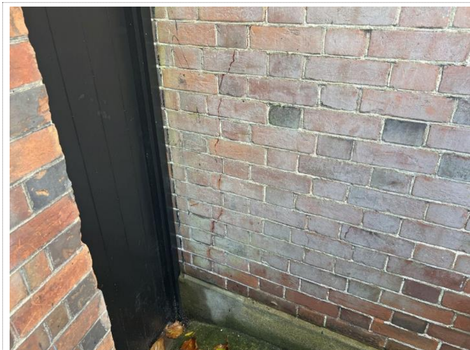
Plate 4. Vertical crack to garage wall.
