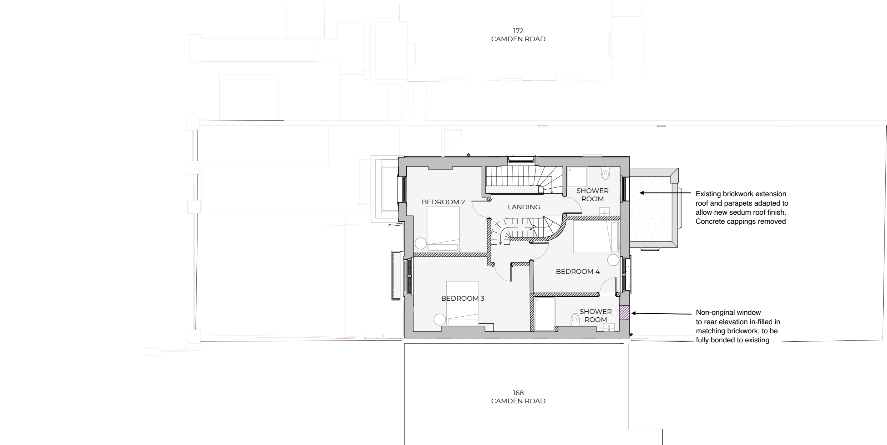
Proposed First Floor
