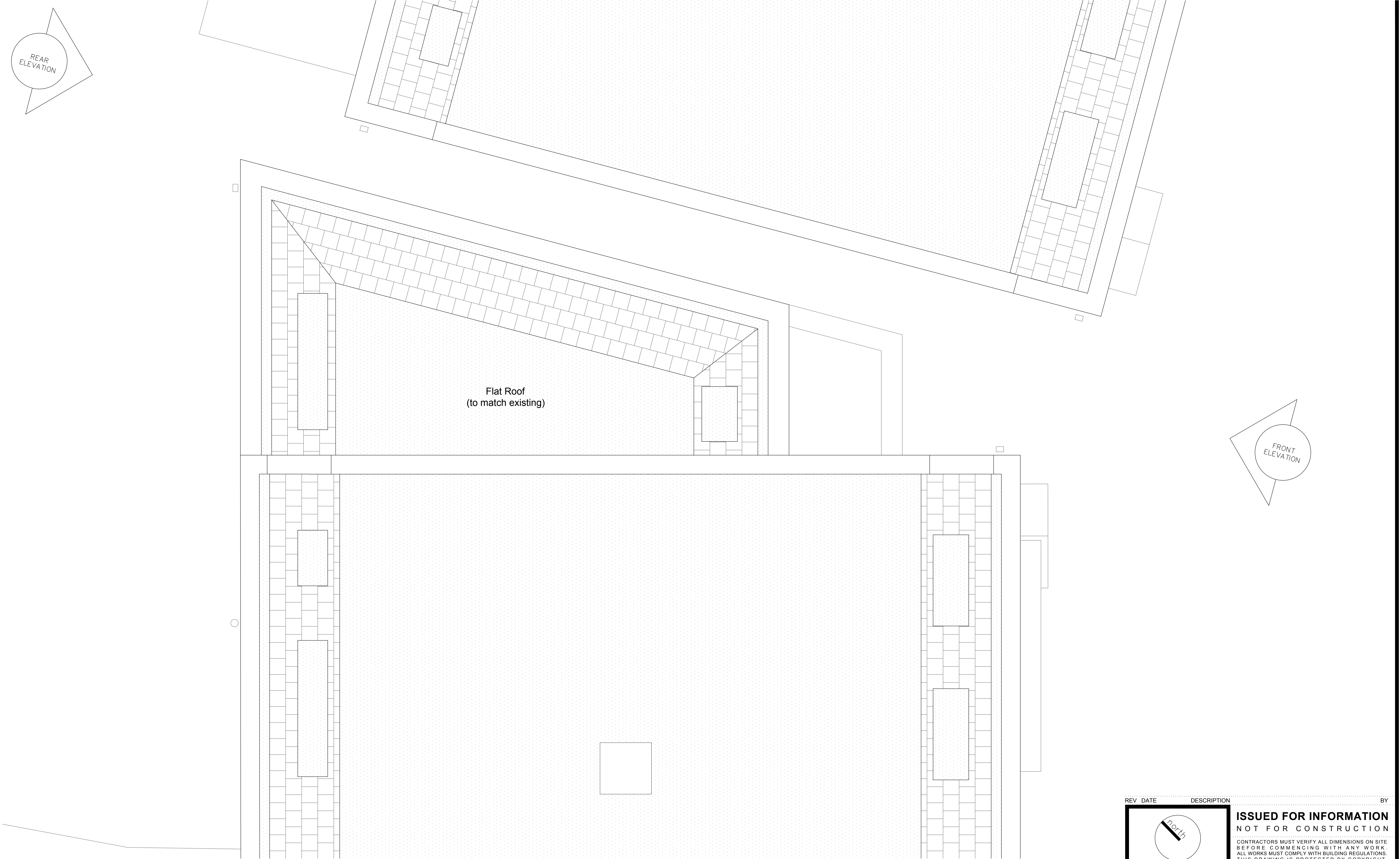
Proposed Roof Plan Scale 1:50@ A3 | 1:25 @ A1 0 1 2
