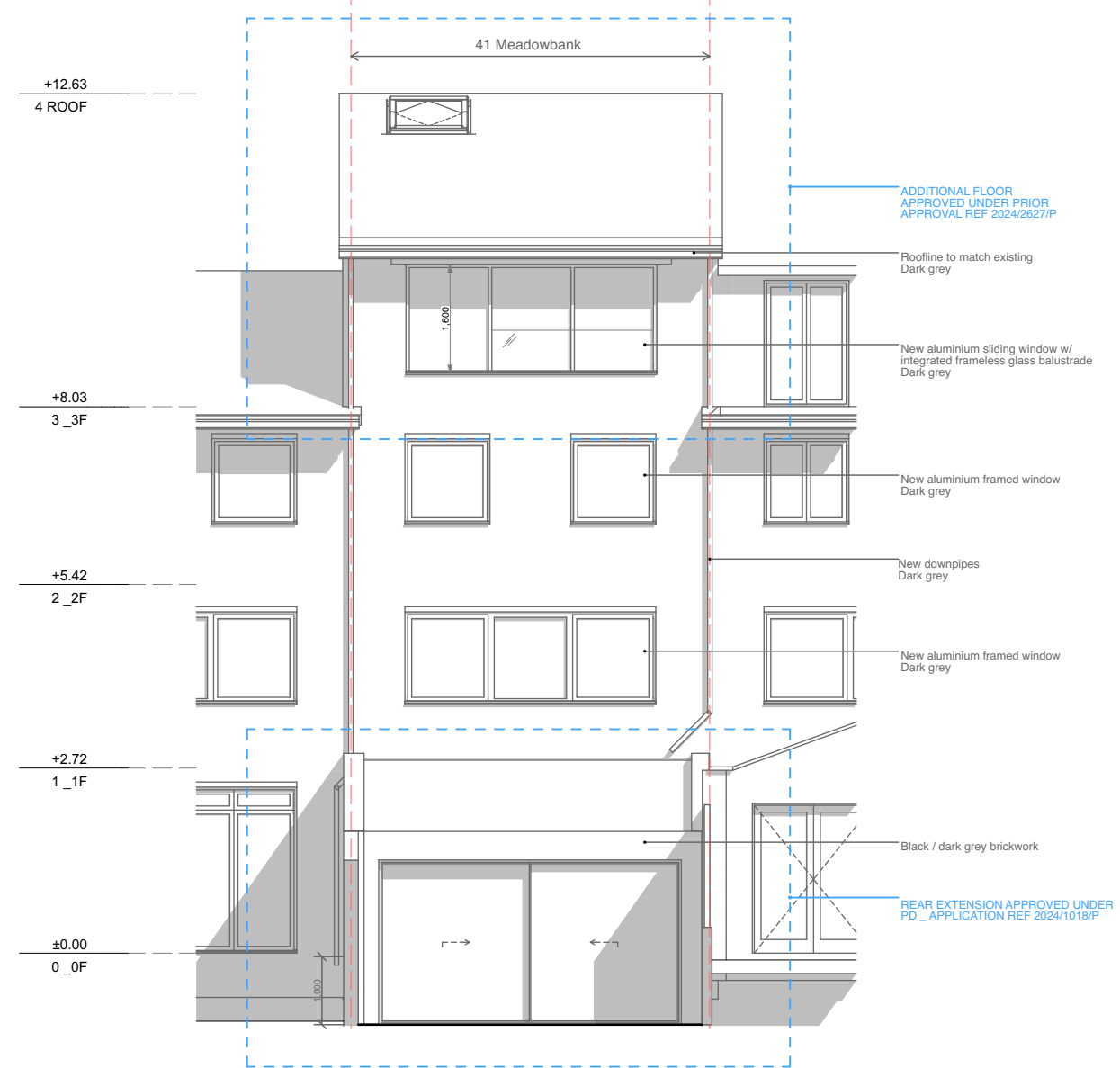
REAR ELEVATION
