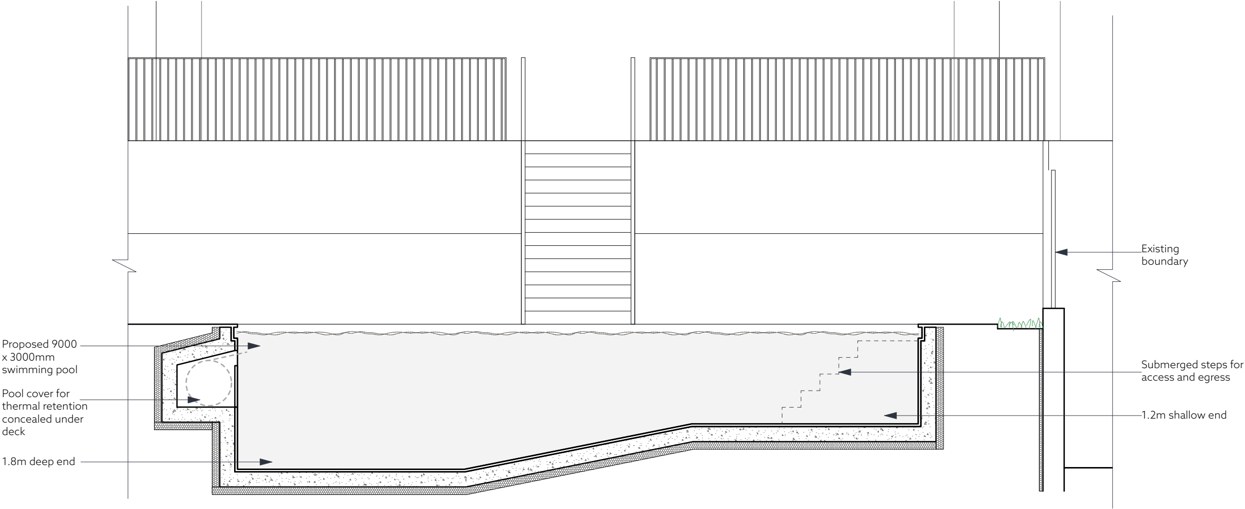
Proposed section A
