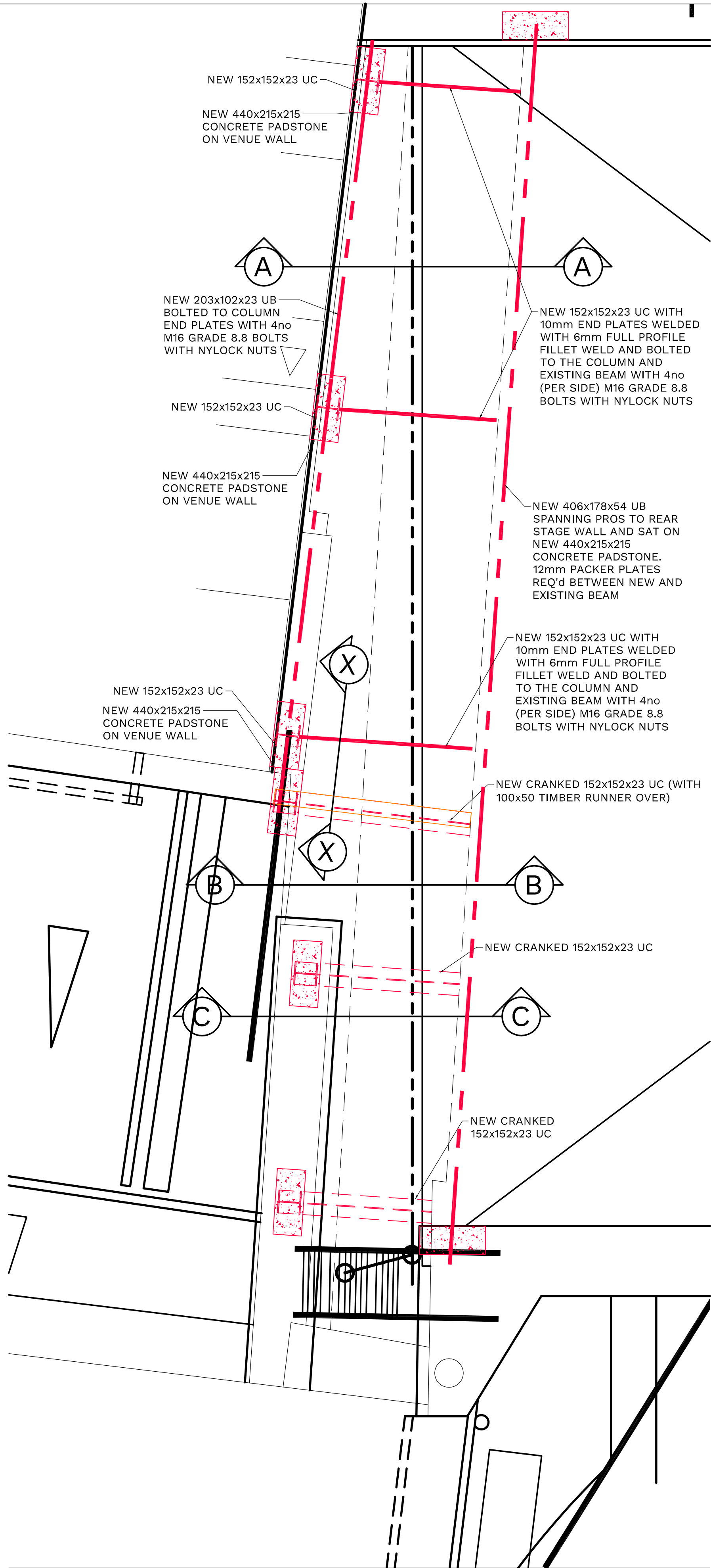
PROPOSED ENLARGED PLAN TO STAGE RIGHT WALL (SCALE 1:20 AT A1)
