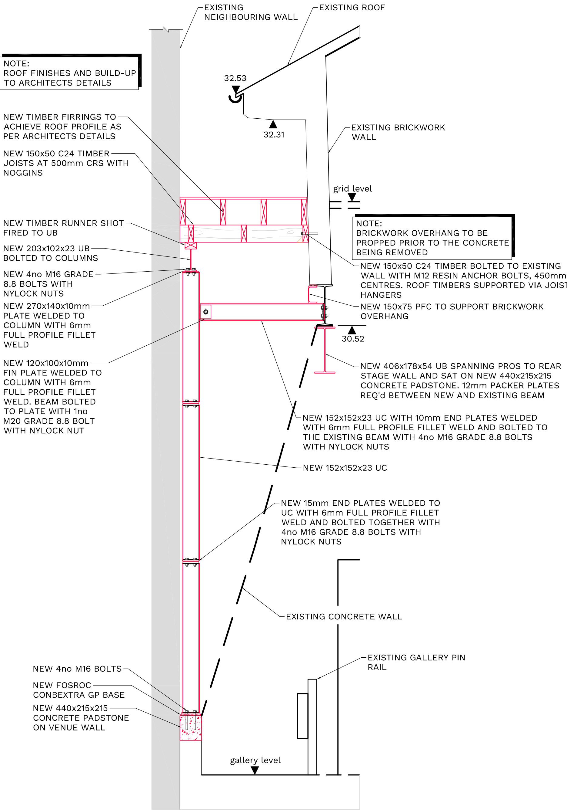
PROPOSED SECTION A-A (SCALE 1:20 AT A1)
