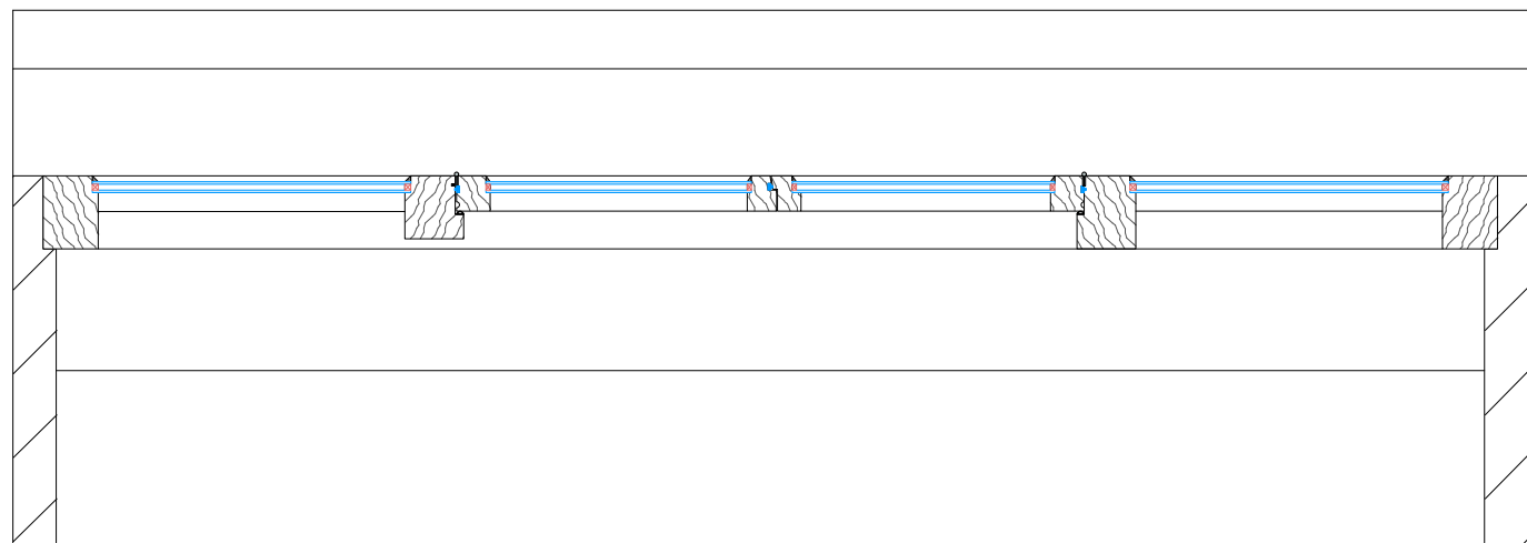
2 Internal window elevation & plan 1:10
