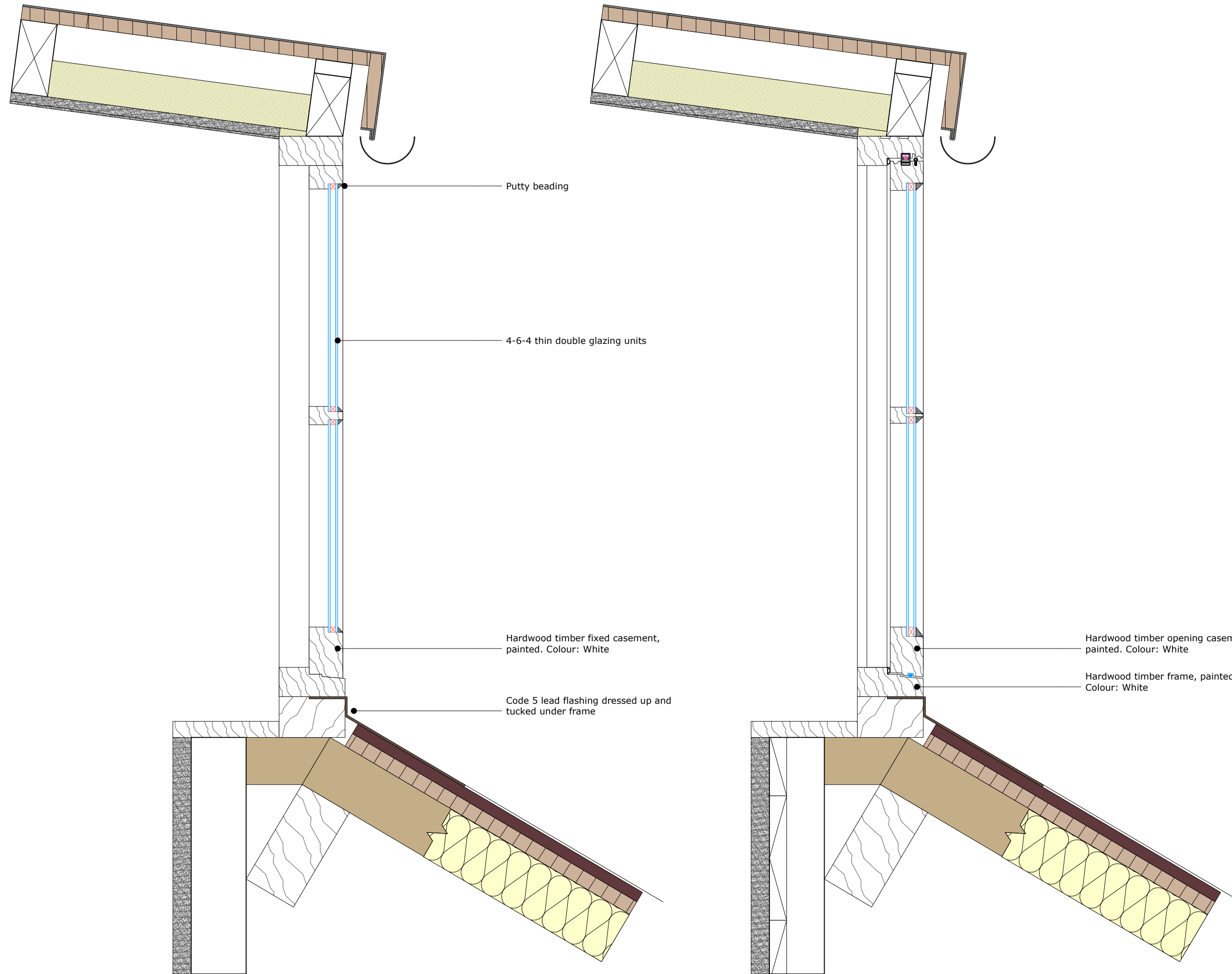
3 Section A 1:5
