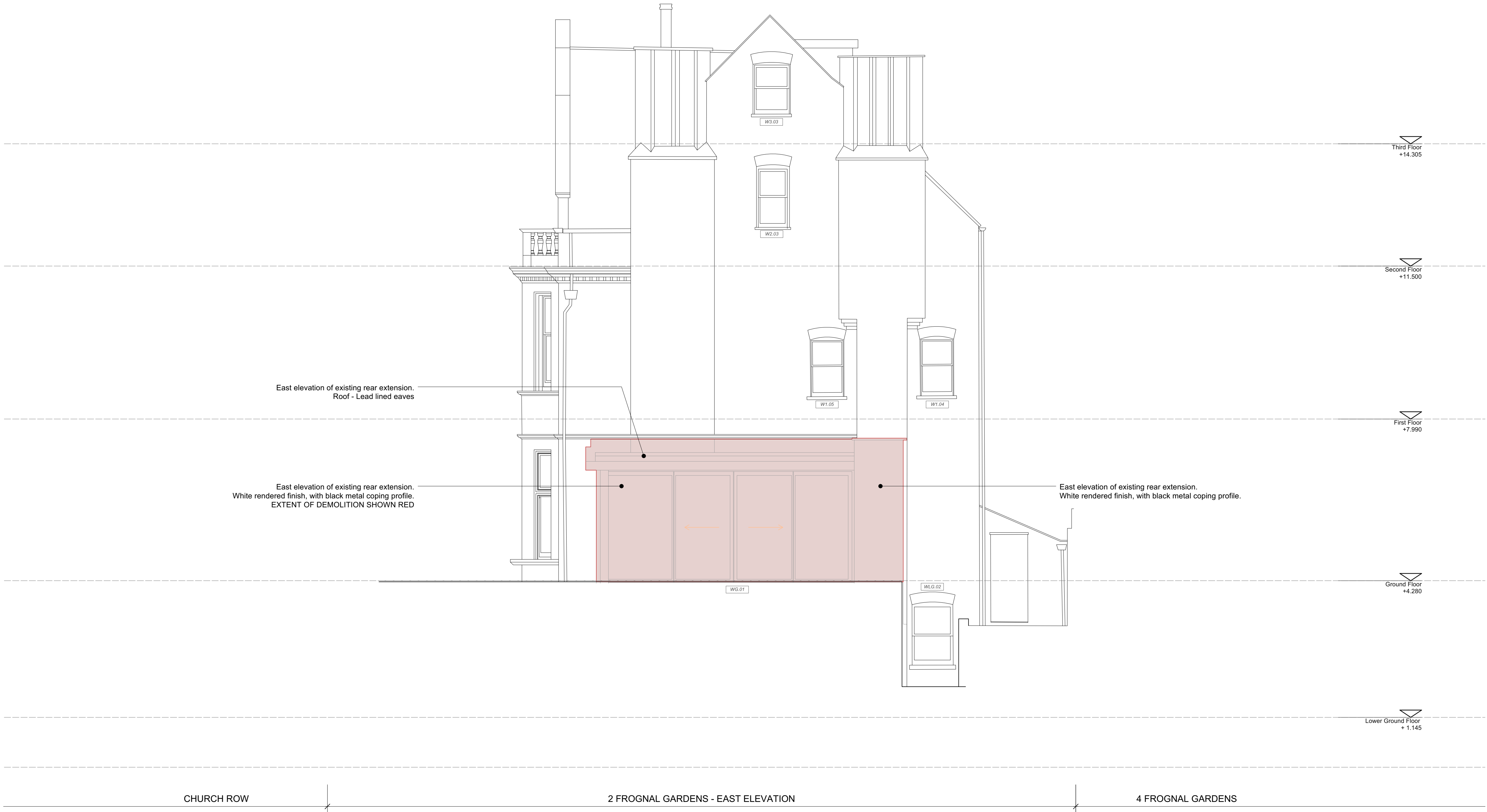
01 Two Frogнал Gardens - existing East Elevation Scale: 1/50
