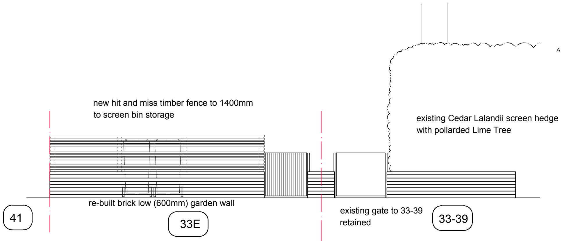
PROPOSED FRONT GARDEN WALL Scale 1:50@A3
