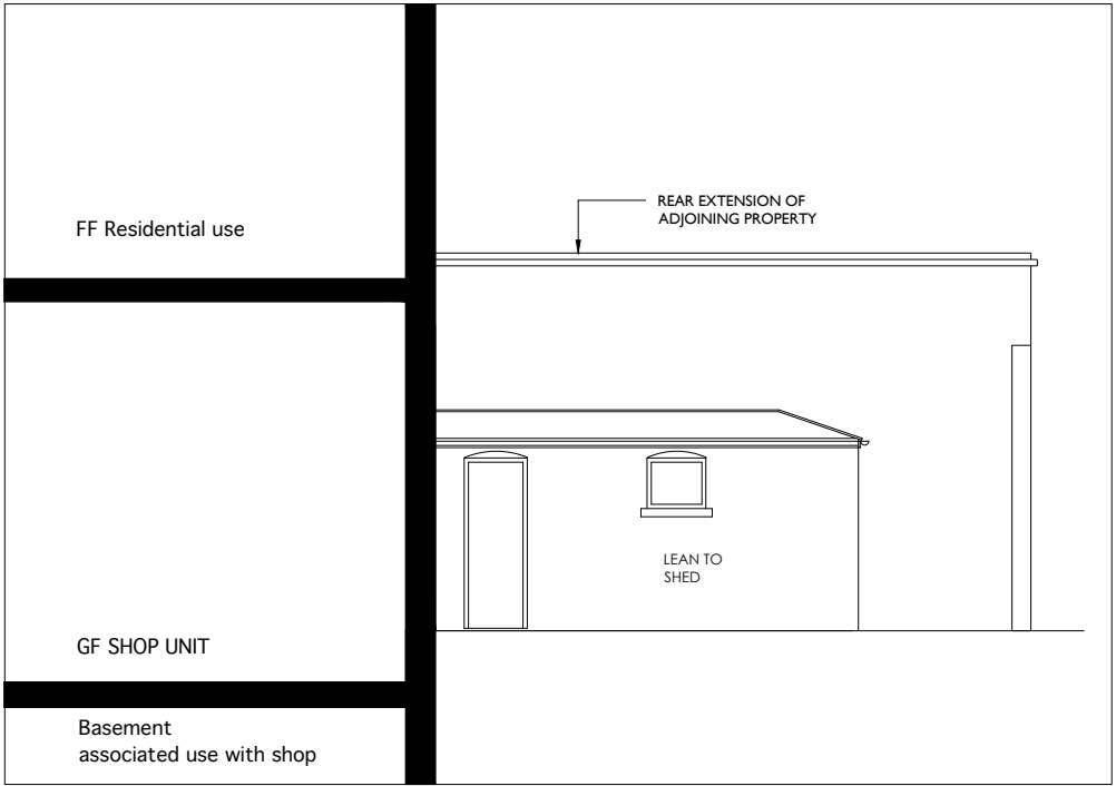
SIDE ELEVATION/ SECTION FACING 42
