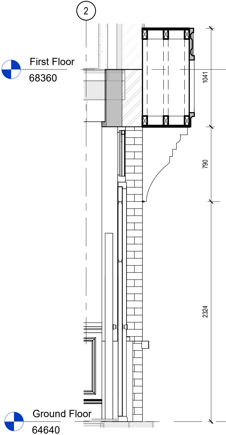
3 External Canopy Section 1 : 25
