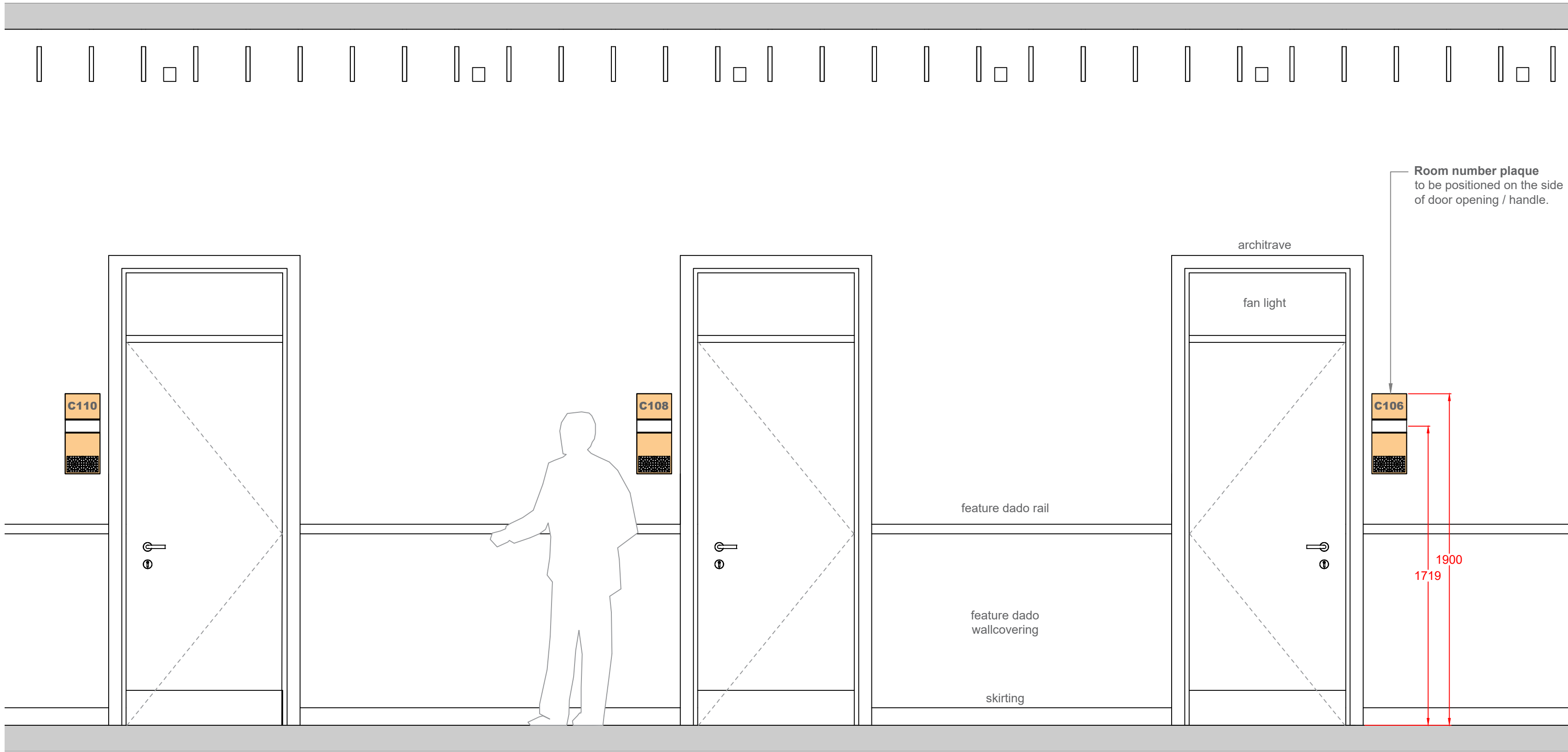
TYPICAL ELEVATION SCALE - 1:20 @ A2
