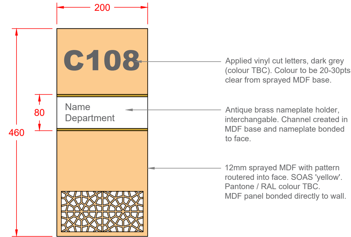
DETAILED ELEVATION SCALE - 1:5 @ A2
