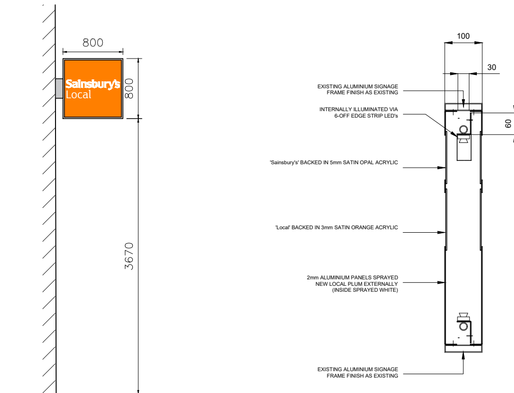
03 PROJECTING SIGN A AND B P199936213 1:50@A3 ILLUMINATION LEVEL - 204 cd/m²
