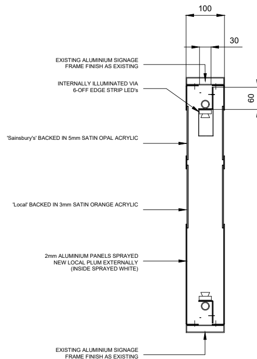
04 PROJECTING SIGN DETAIL A AND B P199936213 1:10@A3
