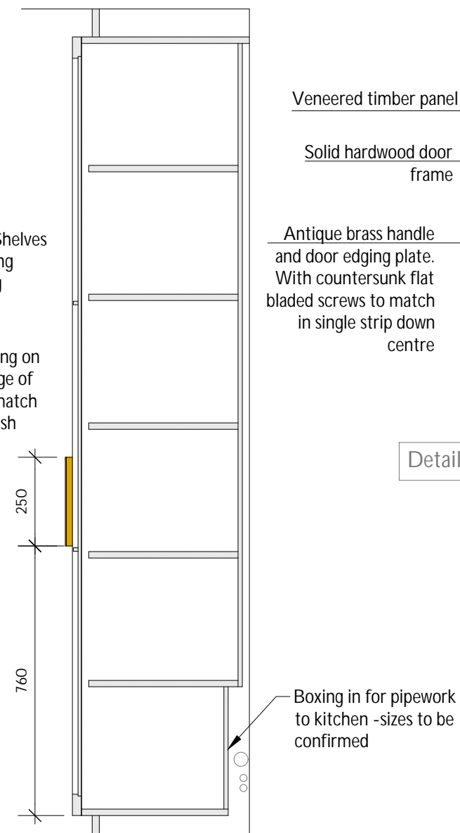
Side Section
