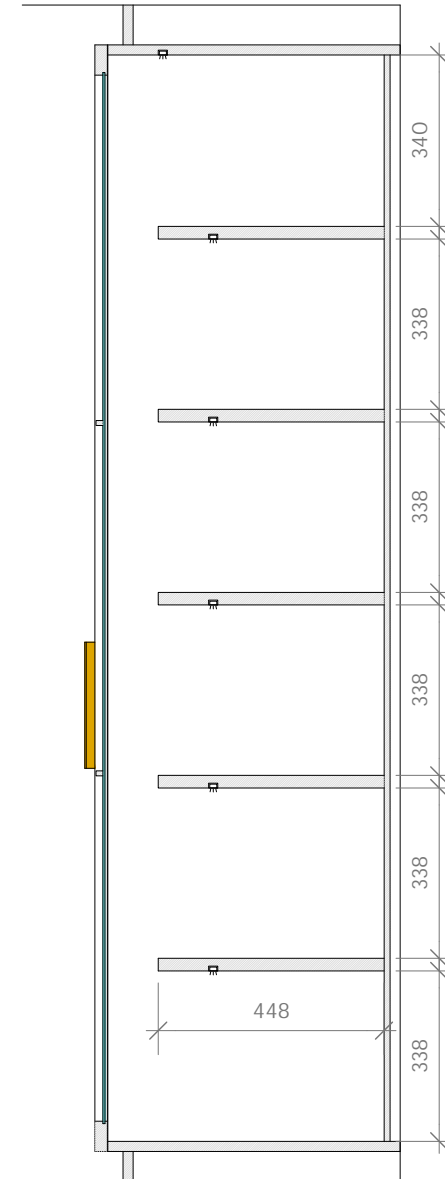
Side Section A
