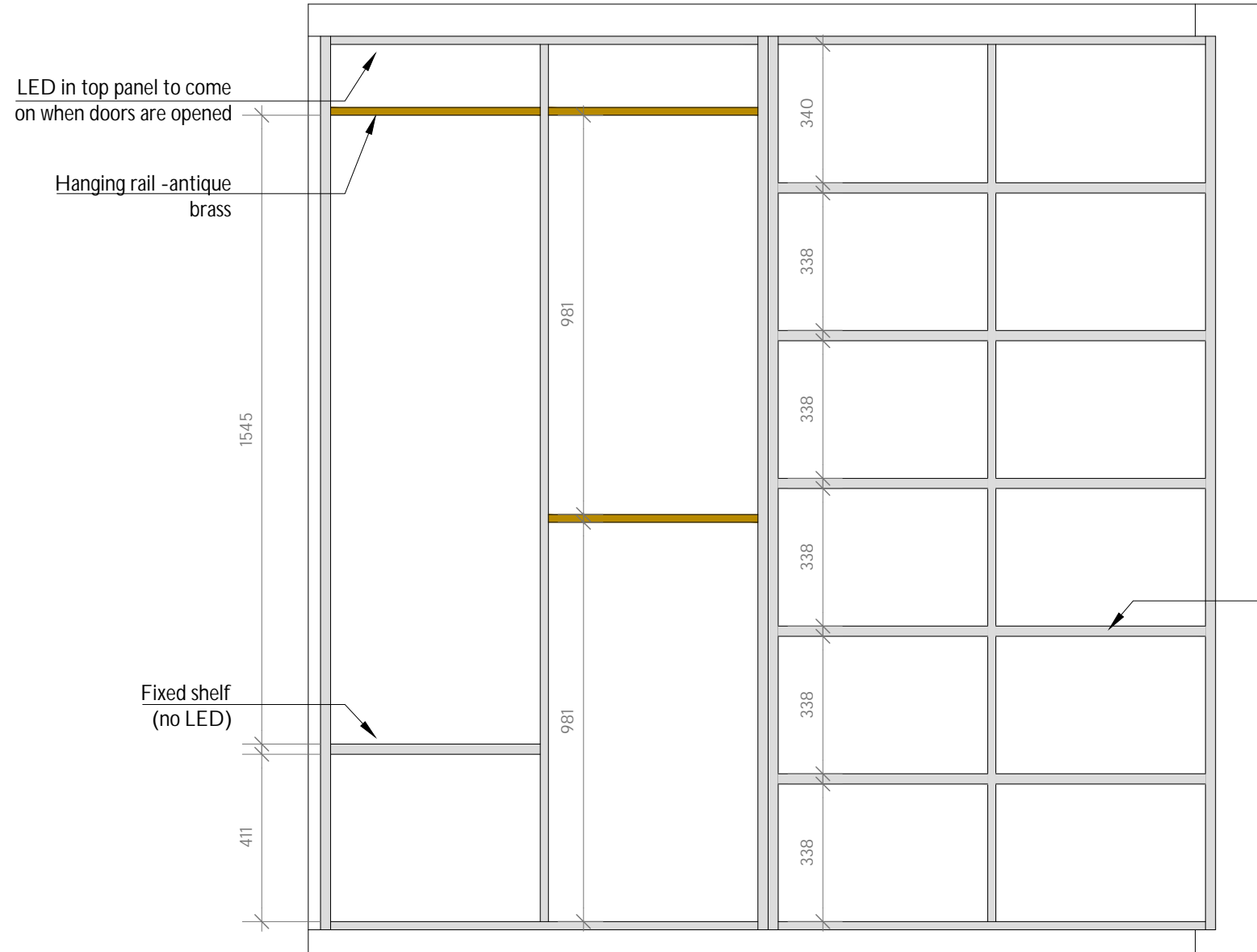
Front - no doors
