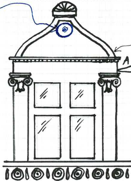
EXISTING UPPER DORMER STRENGTHENING ELEVATION
