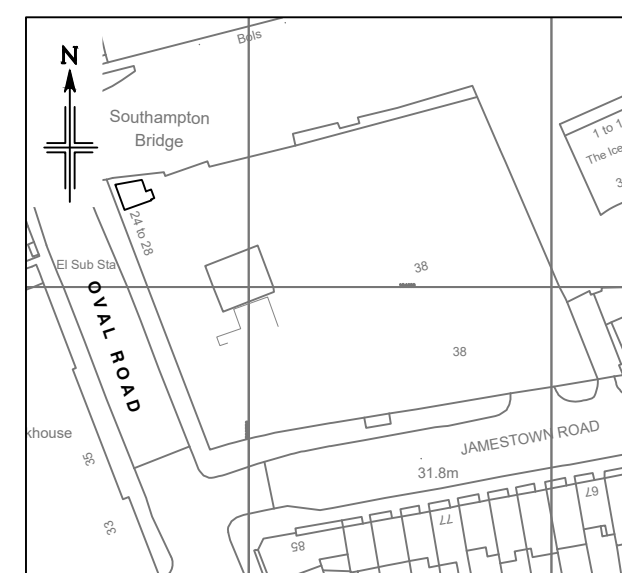
Location Plan Scale 1:1250 This drawing contains Ordnance Survey data which has been reproduced with the permission of the Controller of Her Majesty's Stationery Office, Crown copyright 2019. Licence Number 100022432
