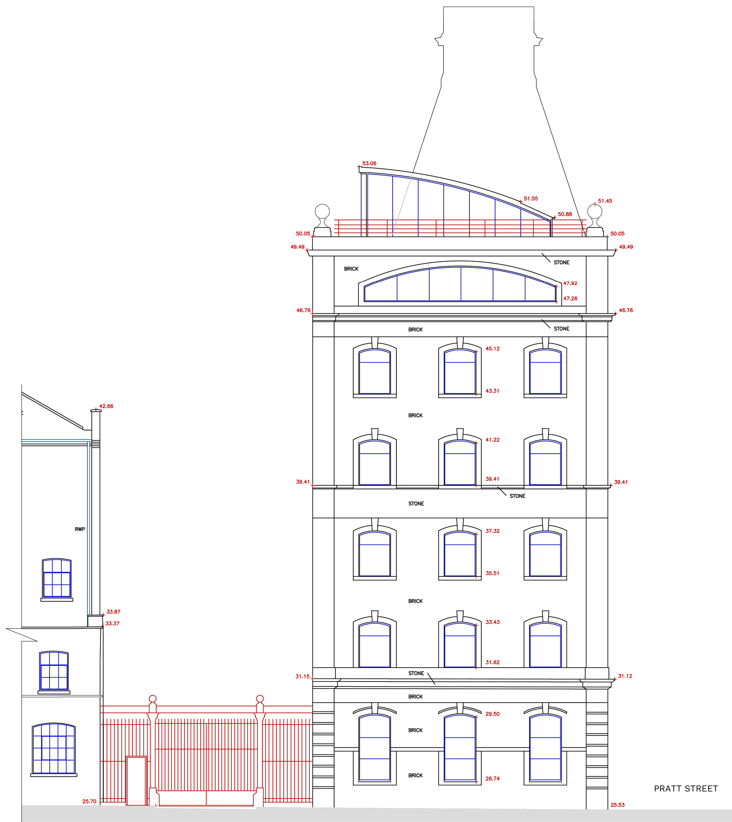
EXISTING MANDELA STREET ELEVATION (SCALE 1:100 AT A1)
