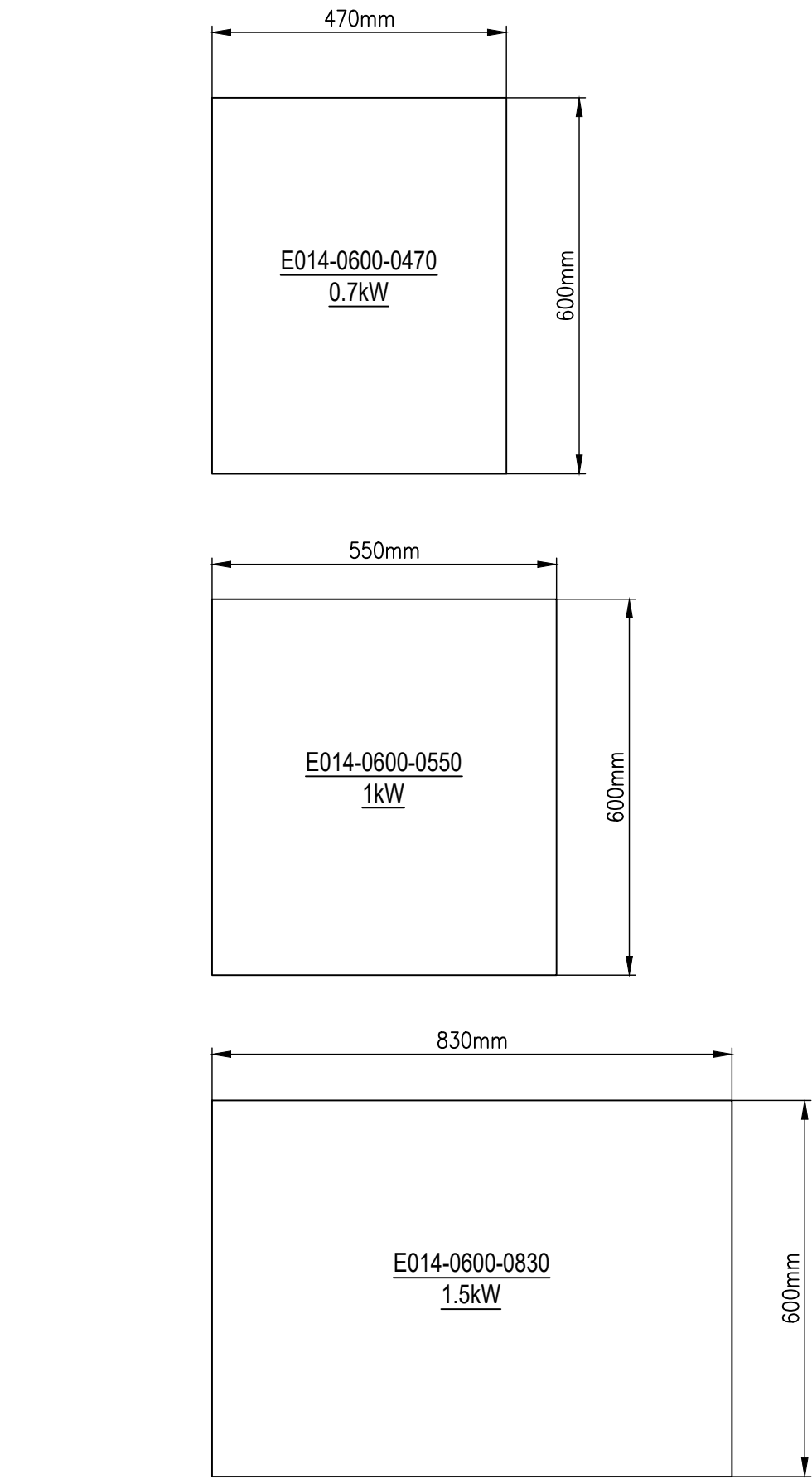
STELRAD ELECTRIC RADIATOR DIMENSIONS
