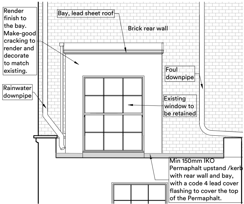
Elevation A (Rear wall of Taviton Annexe) As Proposed
