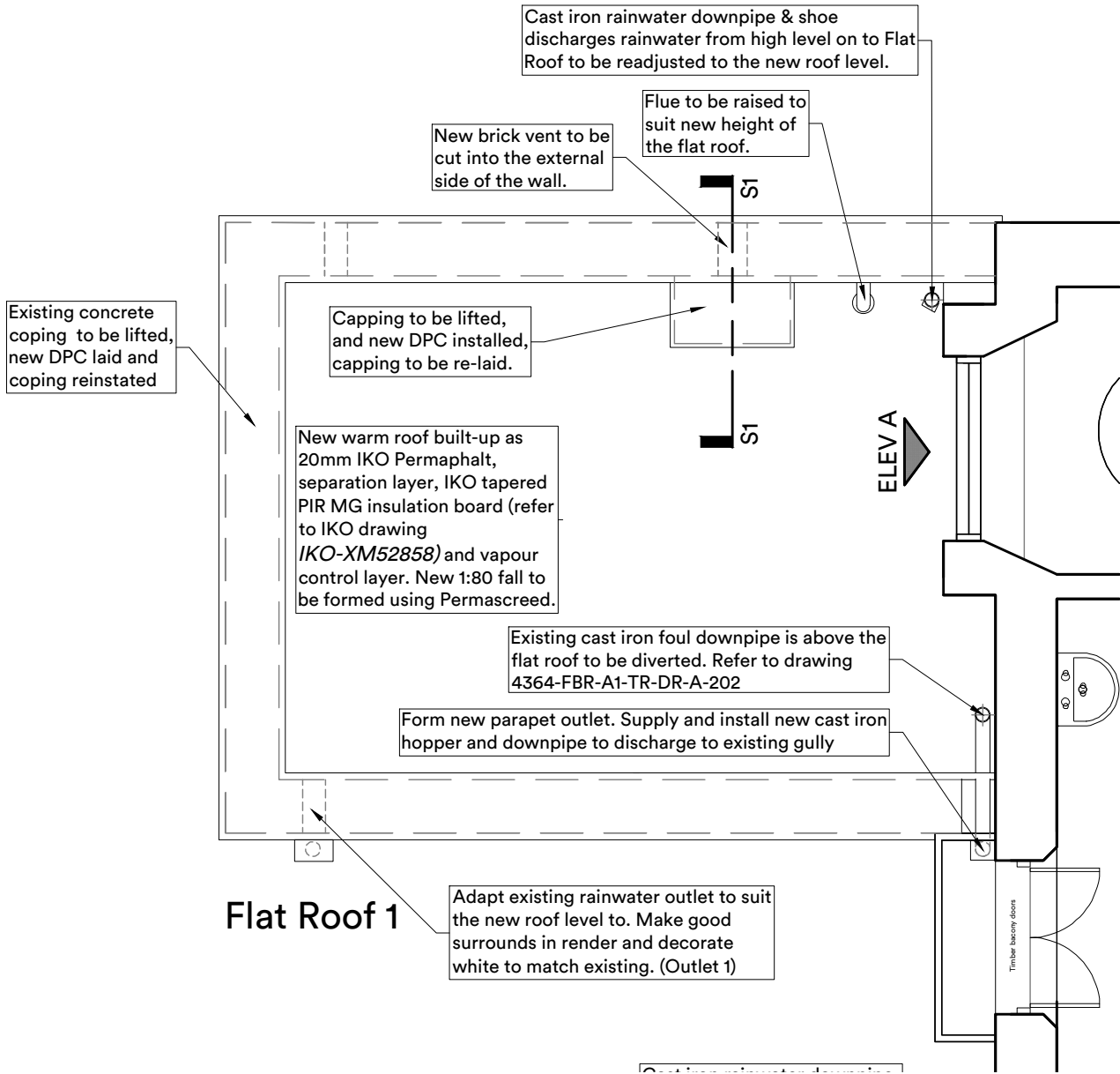
Flat Roof 1 Plan (12 Taviton Street) As Proposed
