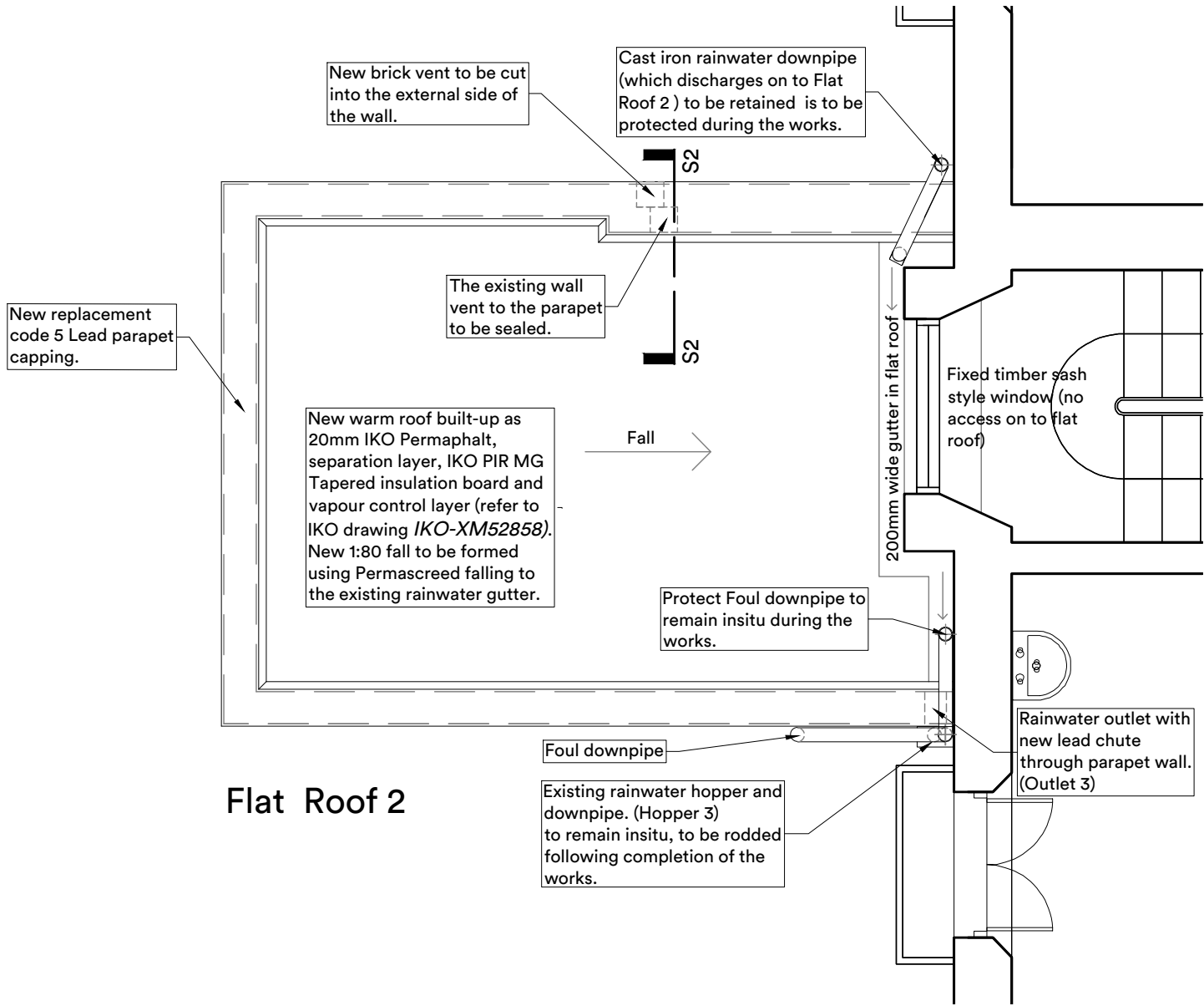
Flat Roof 2 Plan (11 Taviton Street)
