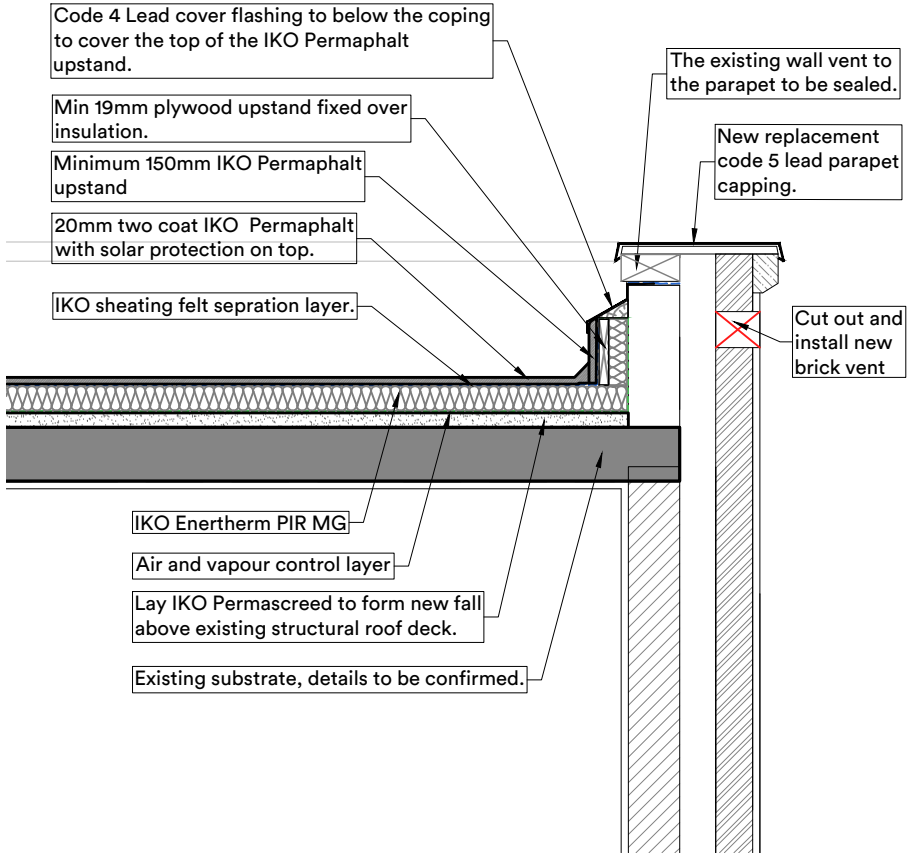
Section S2-S2
