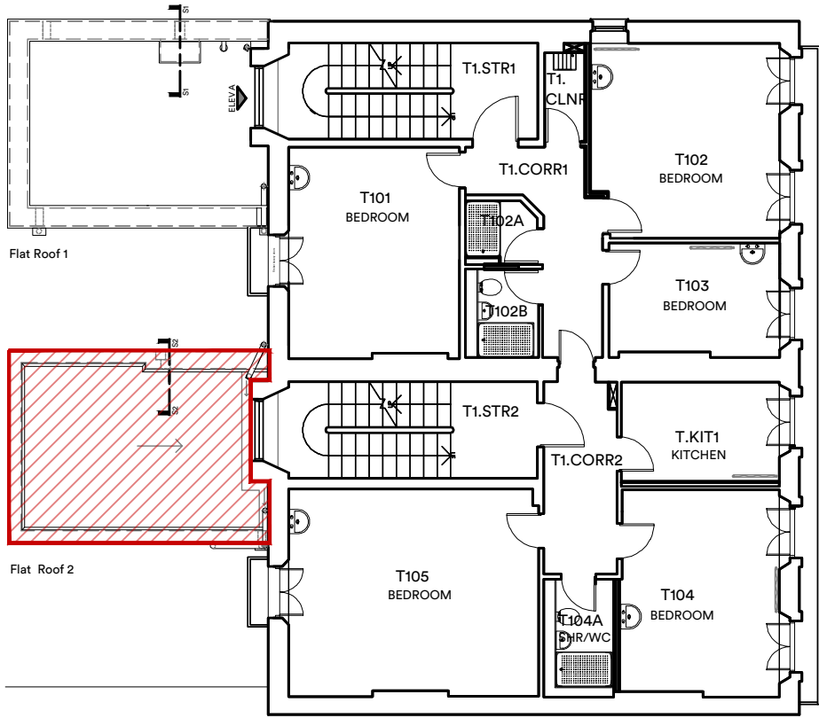
Key Plan
