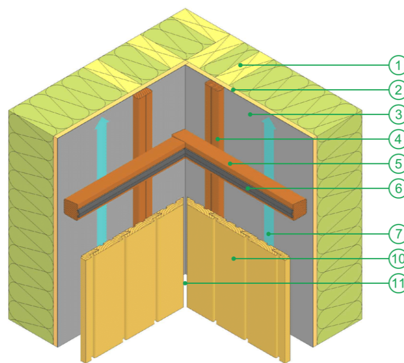
Internal open mitre corner Isometric diagram
