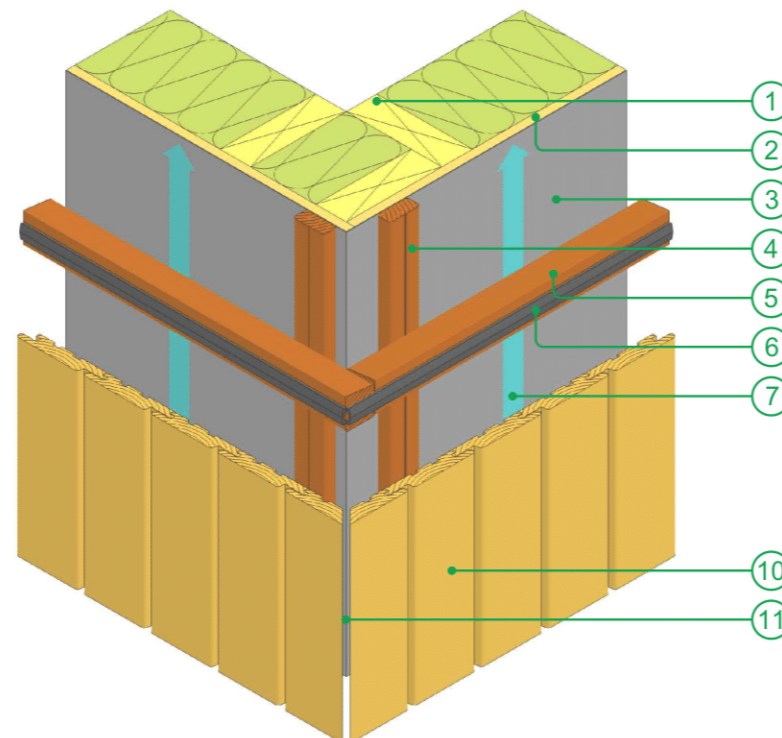
External open mitre corner Isometric diagram
