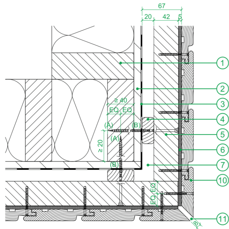
External open mitre corner Plan view (scale 1:4)
