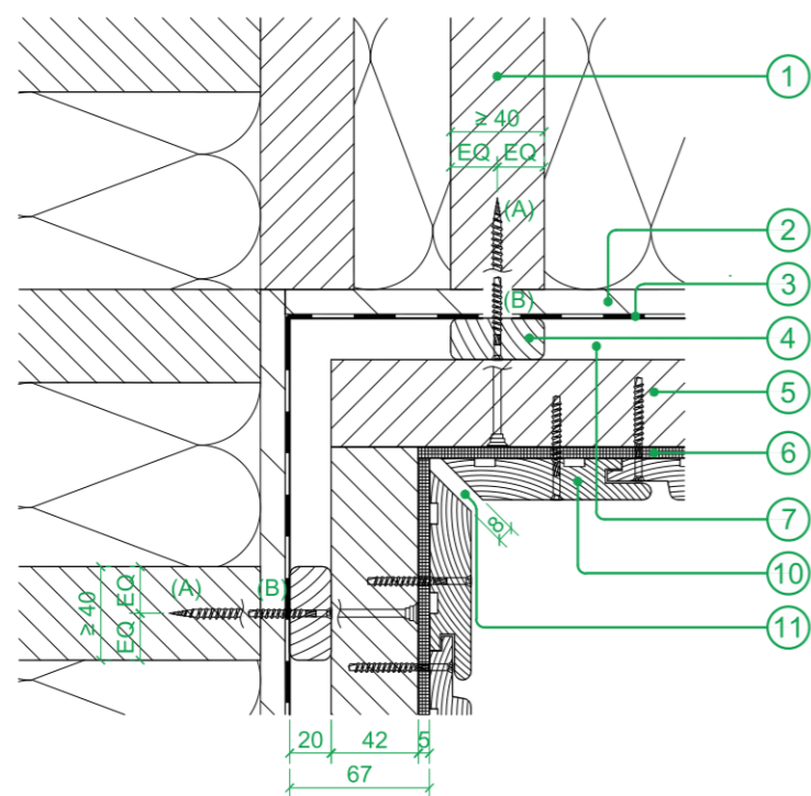
Internal open mitre corner Plan view (scale 1:4)
