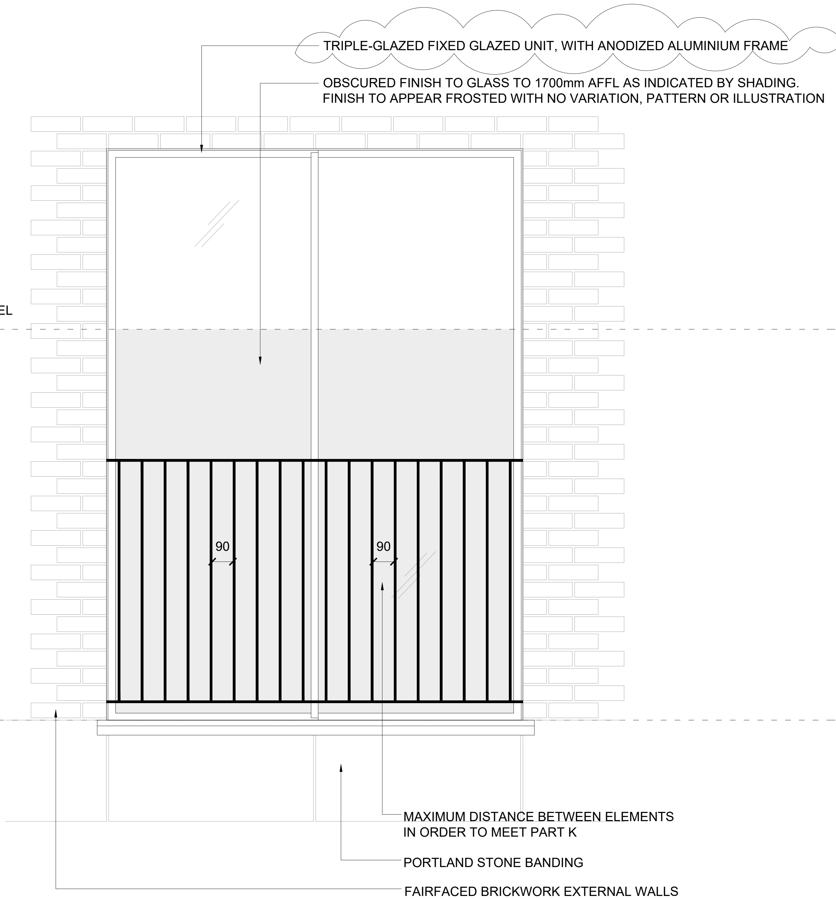
ELEVATION - Typical Window Assembly Type B Showing Aluminium Fins.
