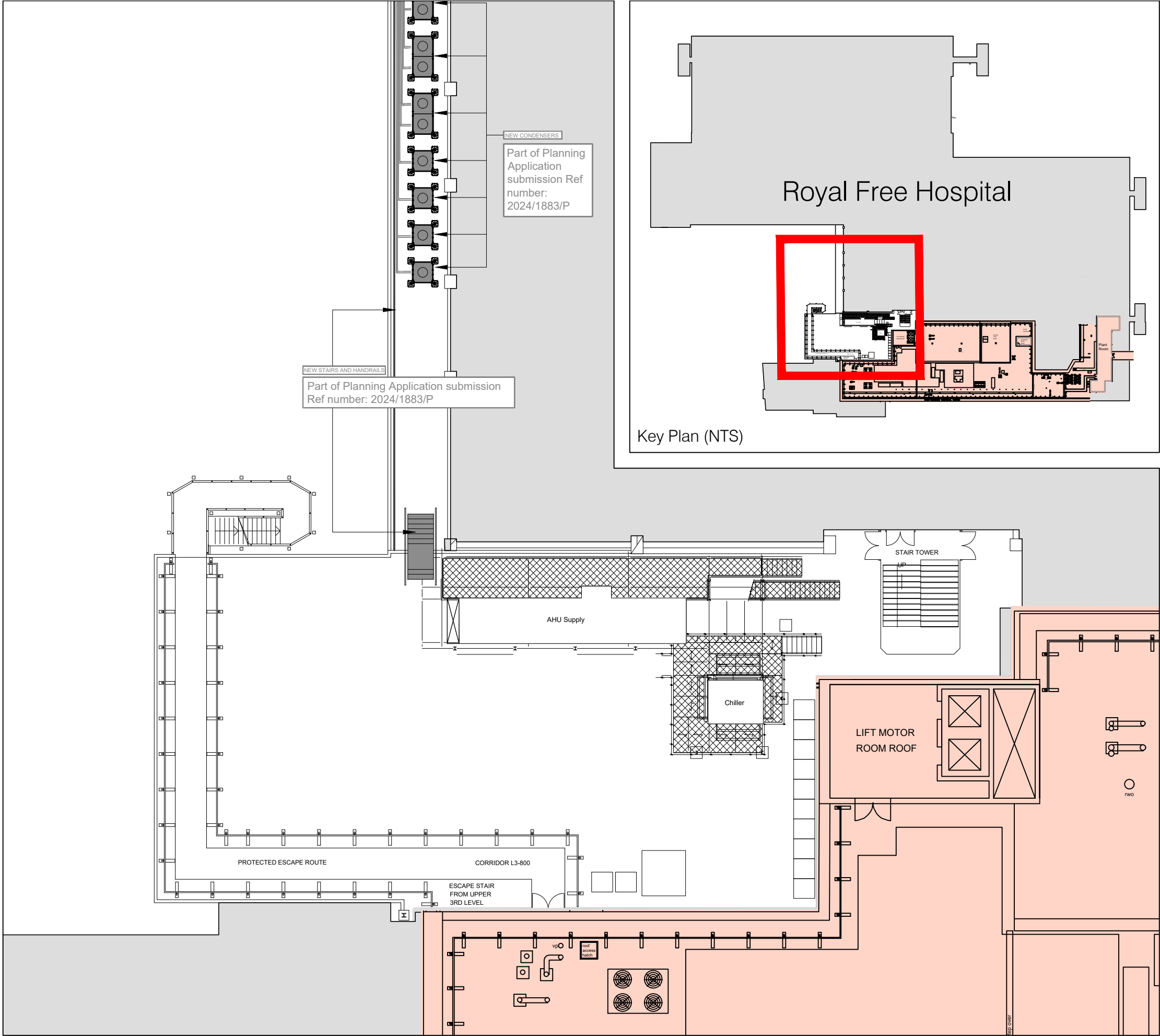
01 Existing 3rd Floor Plan (01)002 1:200 @ A3
