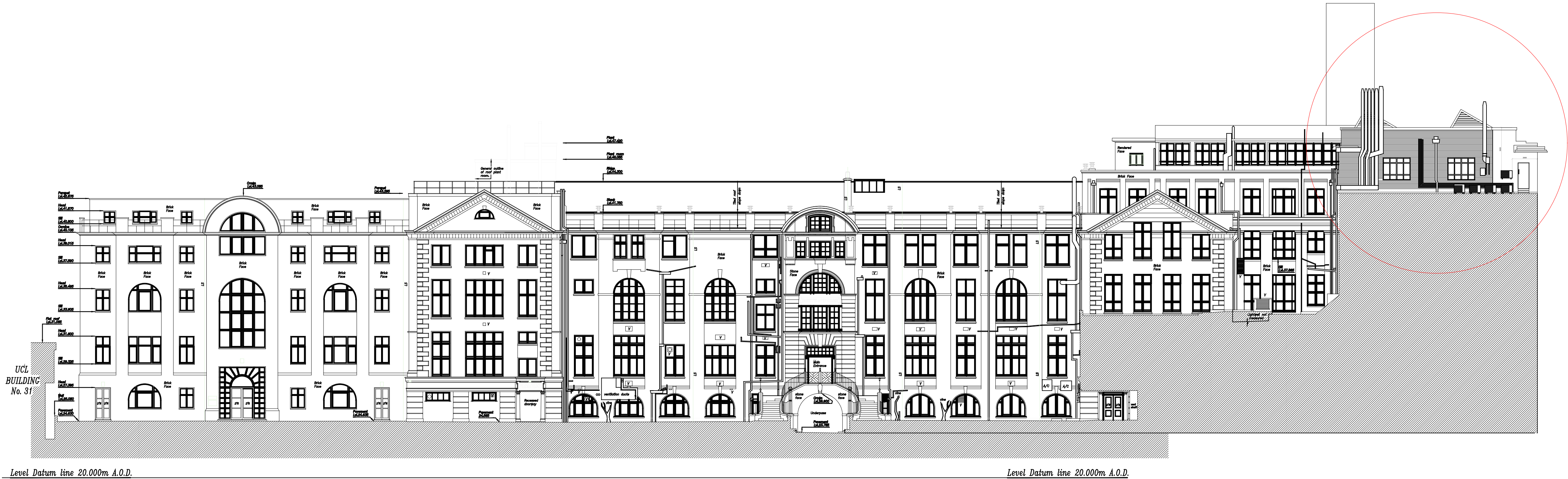
FOURTH FLOOR ELEVATION (NORTH WEST FACING)
