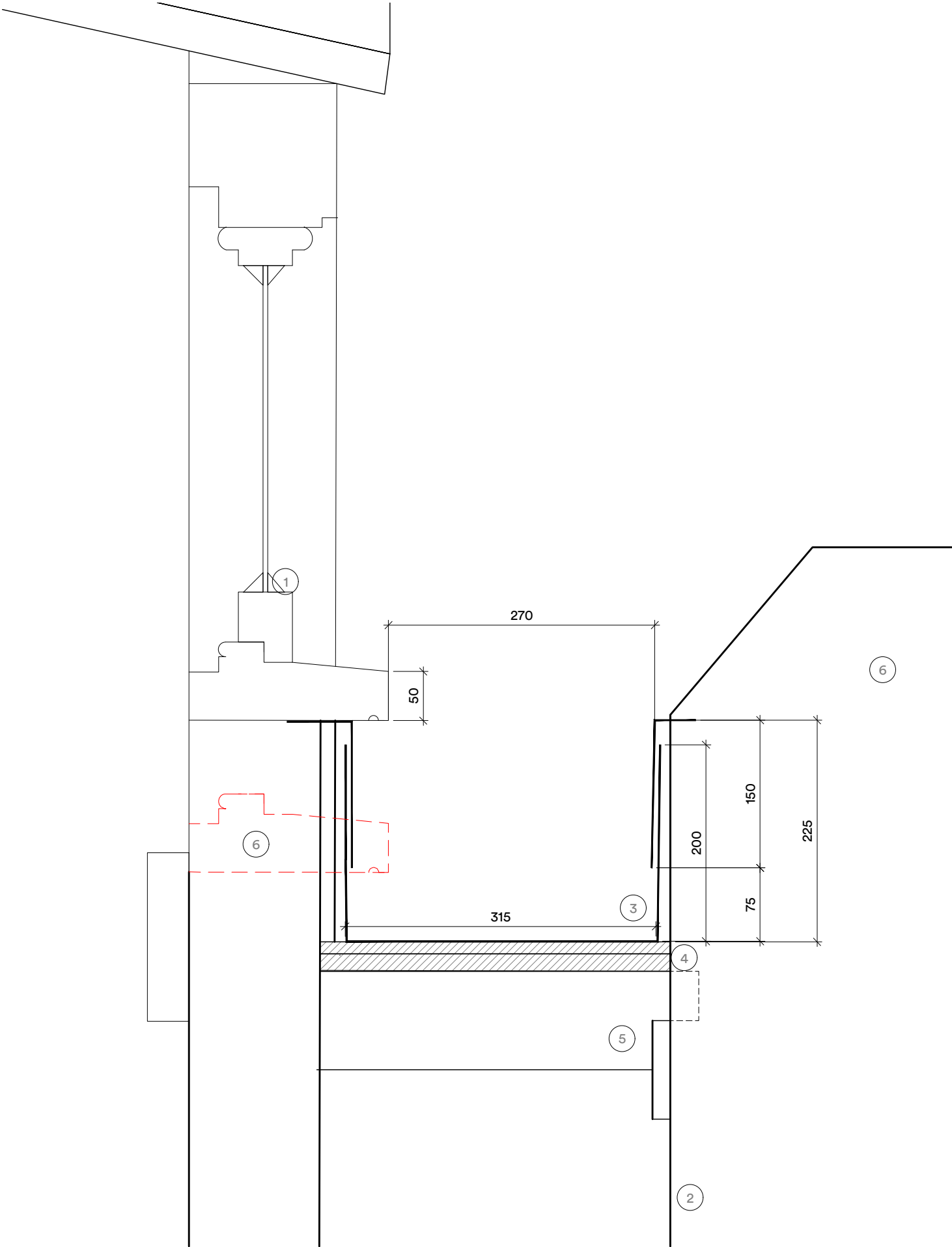
Top of gutter detail outside Store window As Proposed Option 1
