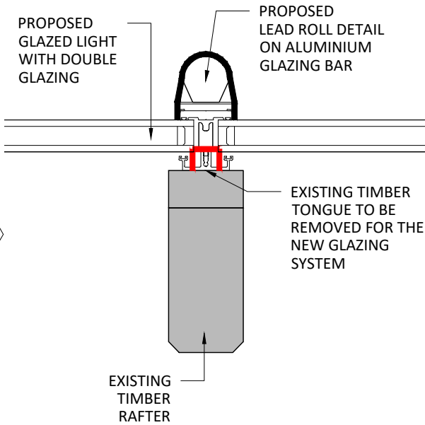
Detail 1 - Typical Glazed Light Detail
