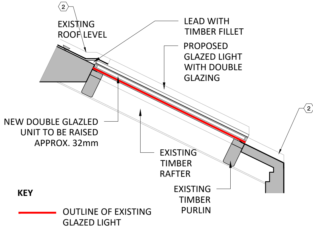
Detail 1 - Typical Glazed Light Detail
