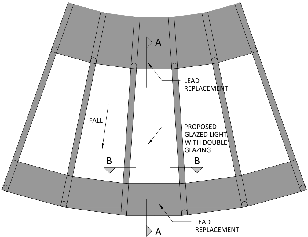
Rotunda Glazed Light Typical Detail
