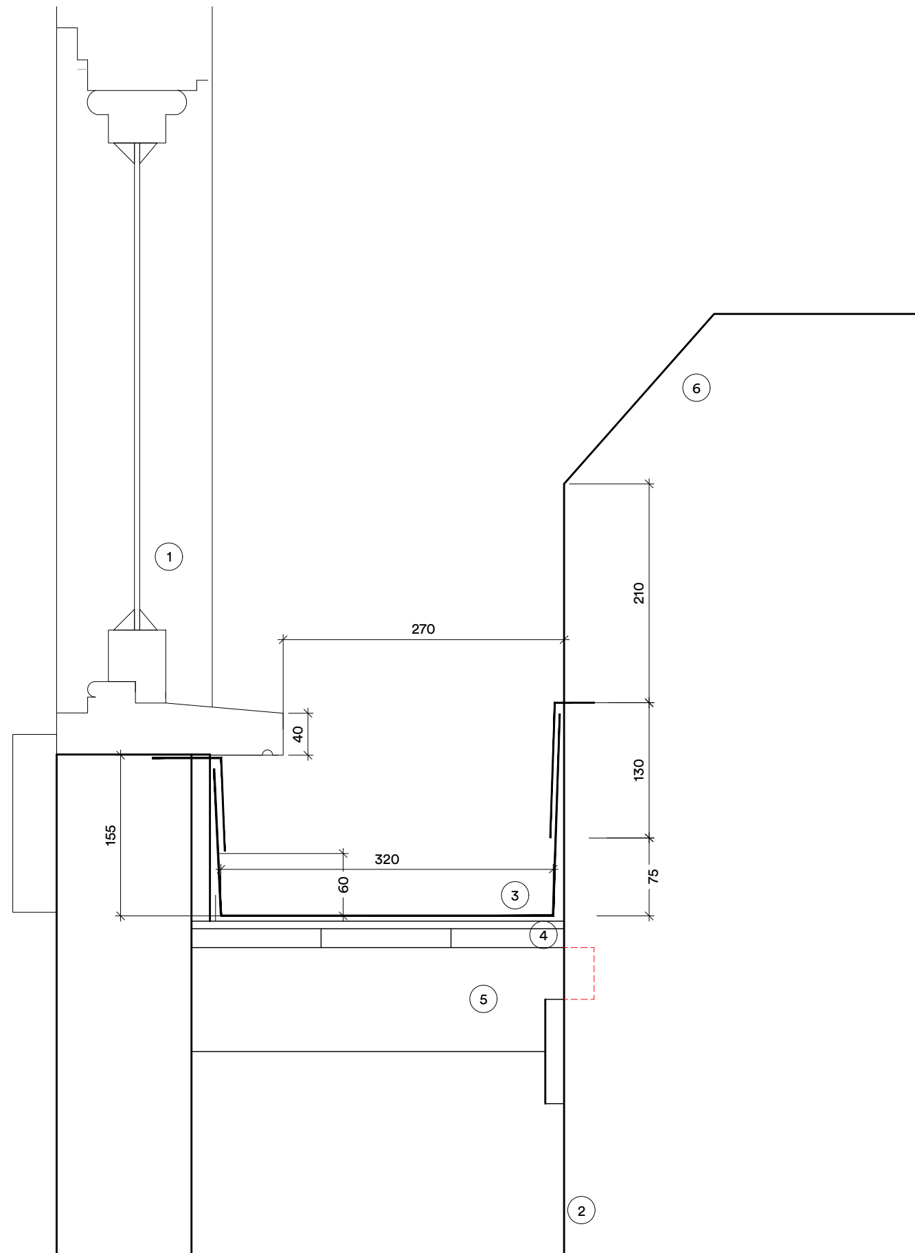
Bottom of gutter detail outside Theatre Office window
