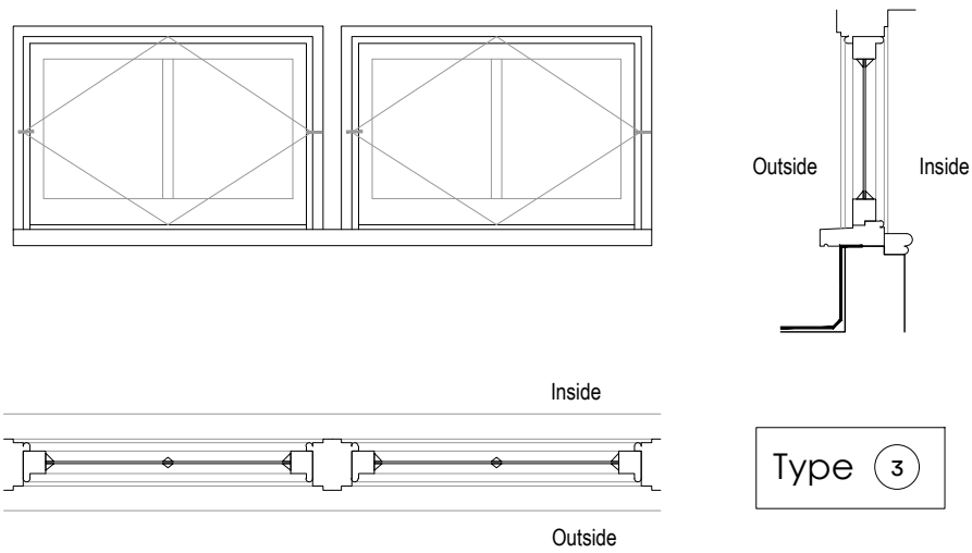
Timber Clerestorey Window Type 3 As Existing 1:20
