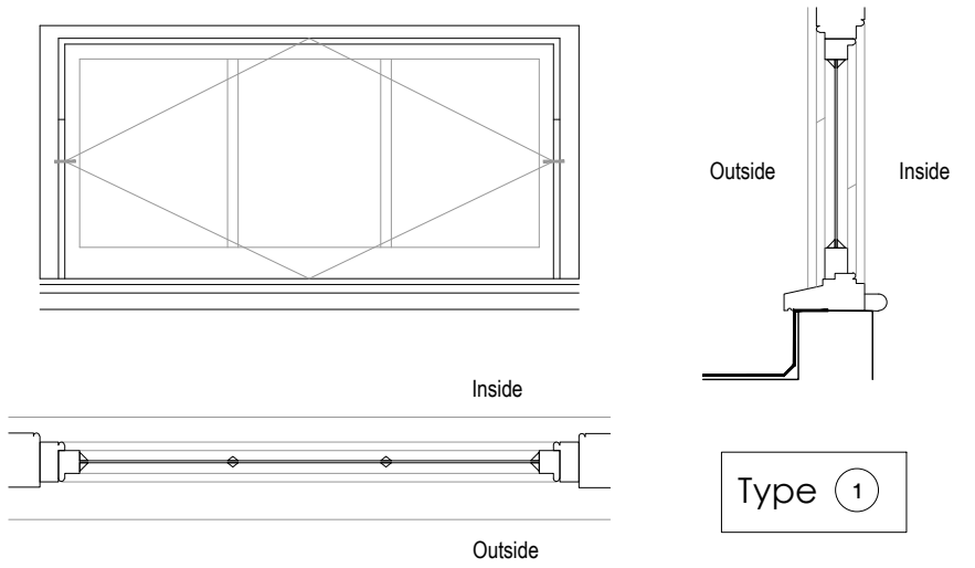
Timber Clerestorey Window Type 1 As Existing 1:20
