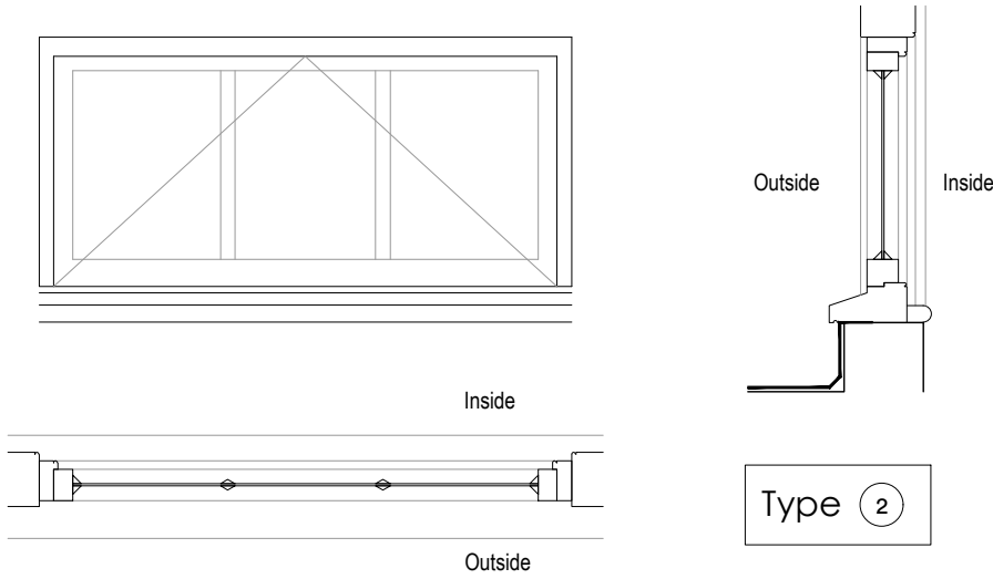
Timber Clerestorey Window Type 2 As Existing 1:20
