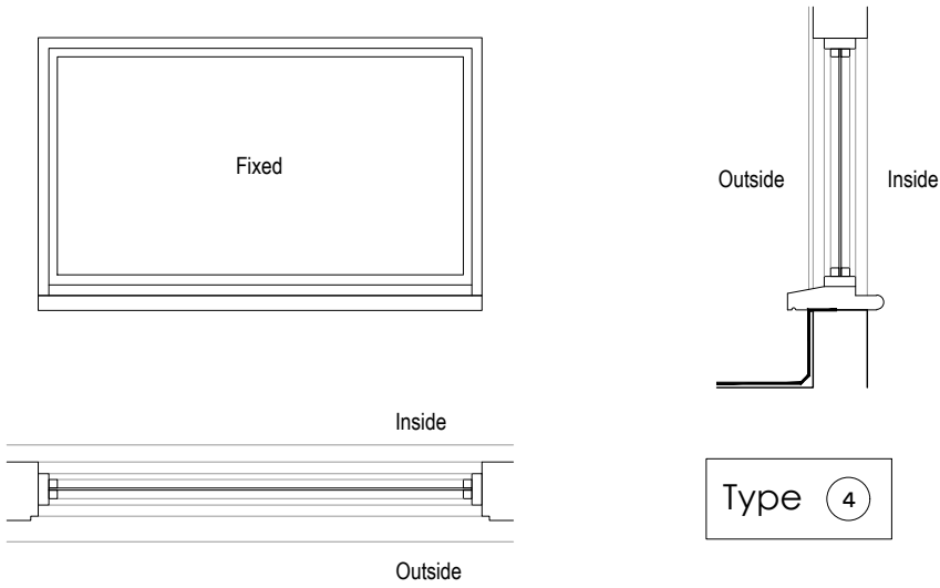
Timber Clerestorey Window Type 4 As Existing 1:20
