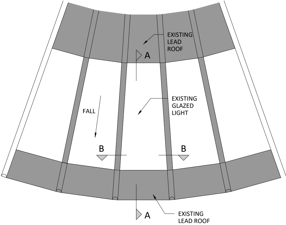
Rotunda Glazed Light Typical Detail
