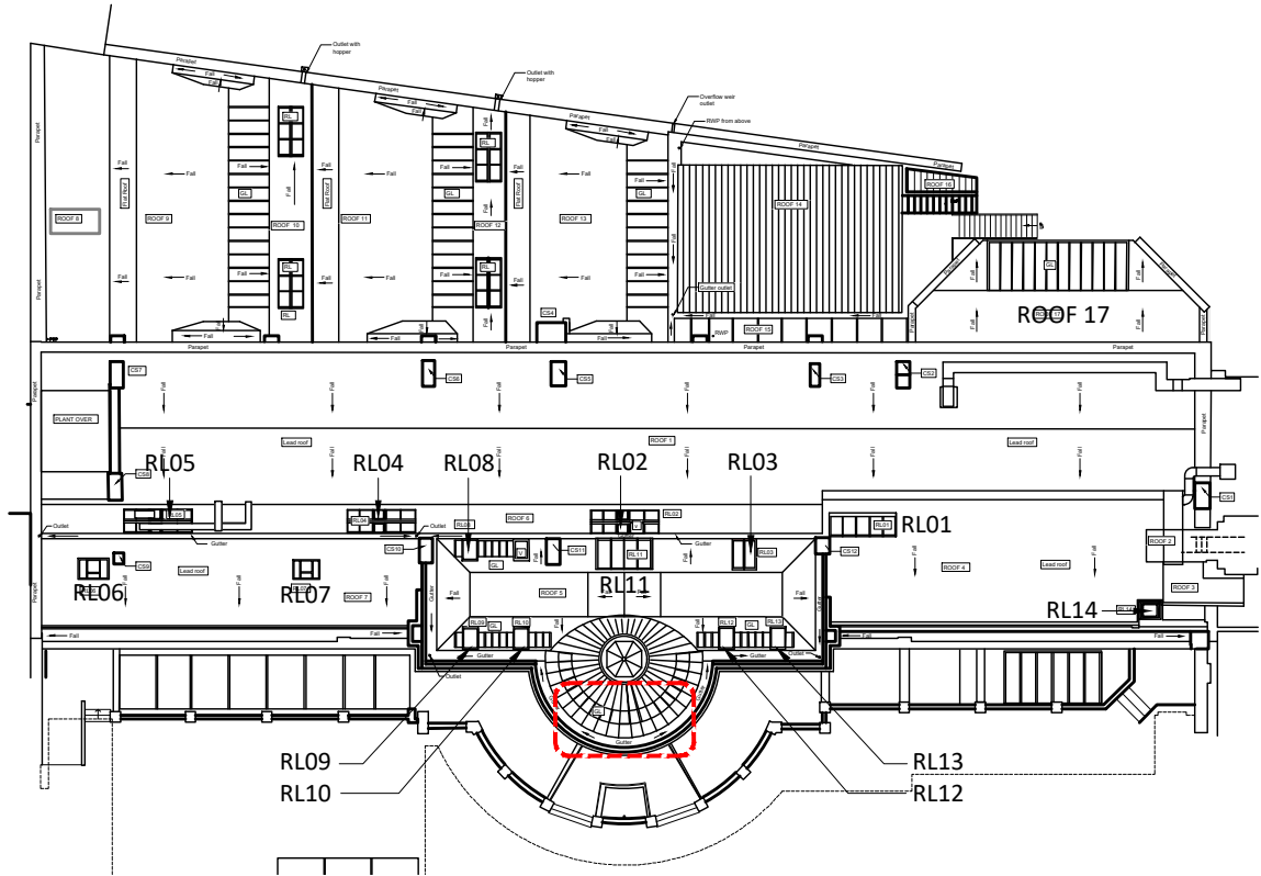
Rooflight Location Plan
