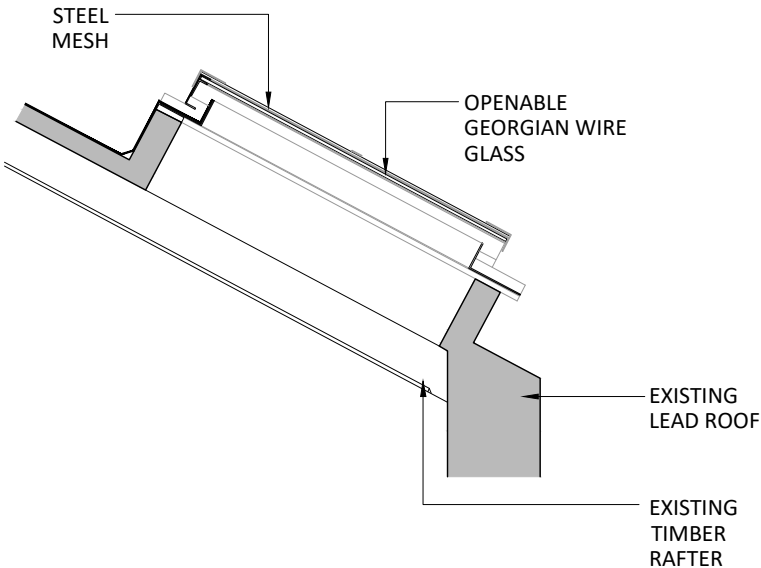
Section A-A As Existing 1:20
