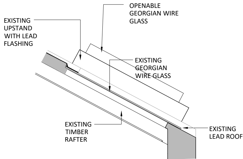
Section C-C with Elevation 1 behind As Existing 1:20
