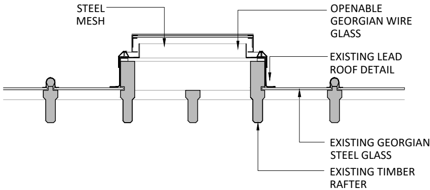
Section B-B As Existing 1:20
