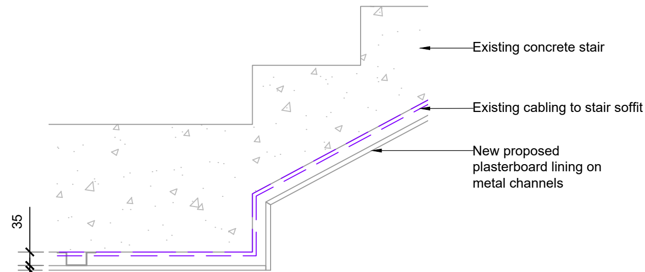
Existing condition 2) - No step in stair landing soffit
