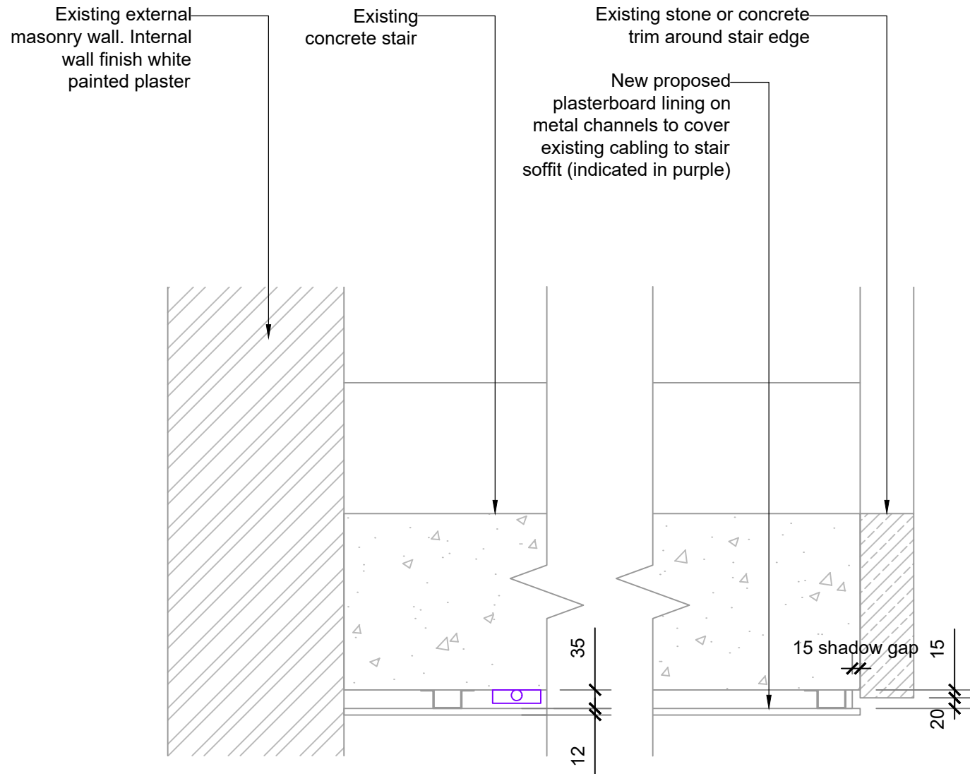
Typical Stair Short Section 1:10 @ A3
