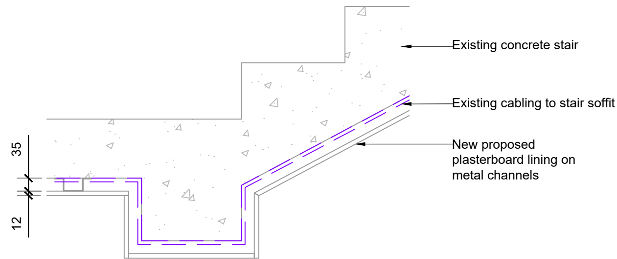
Existing condition 1) - Step in stair landing soffit
