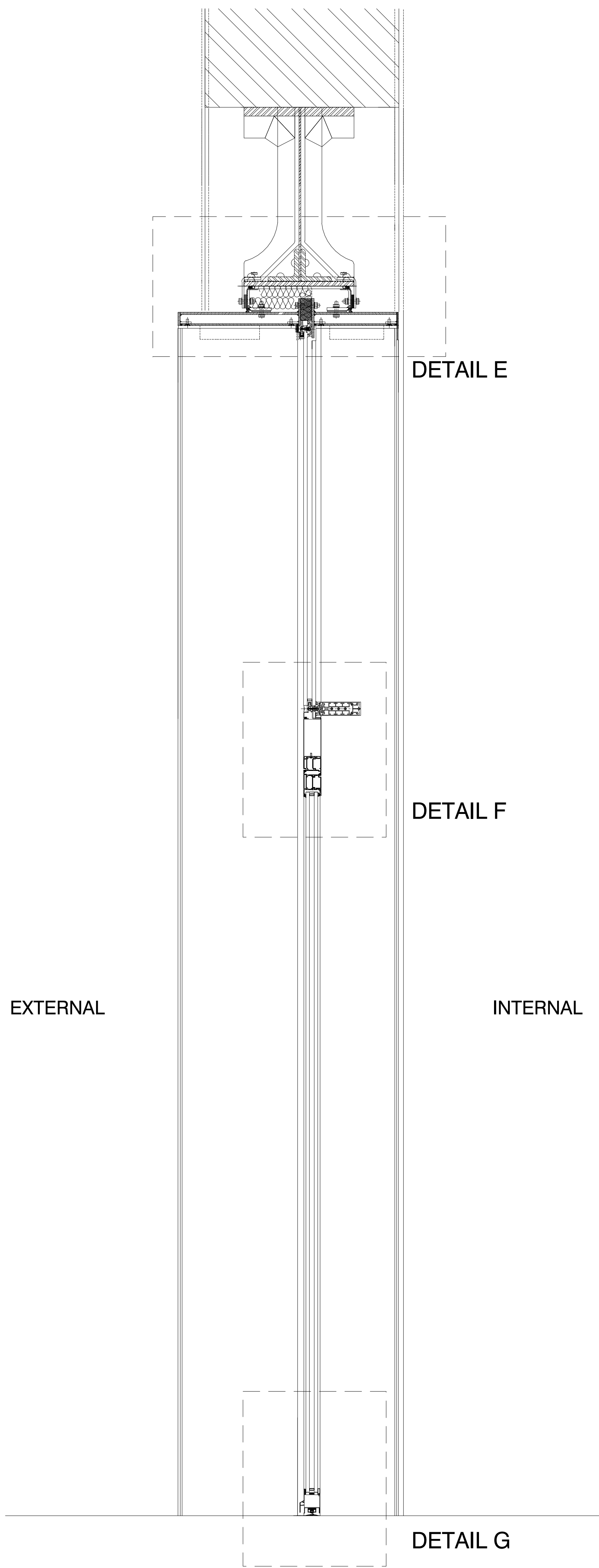
2 DETAILED SECTION OF PROPOSED DOOR 1 : 10
