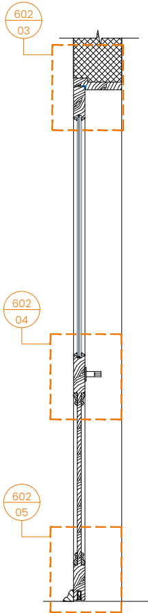
[ 02 ] DOOR SECTION
