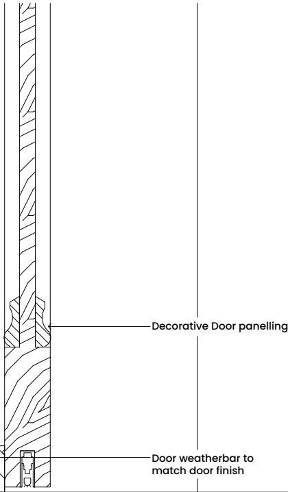
[ 05 ] SECTION - BOTTOM RAIL
