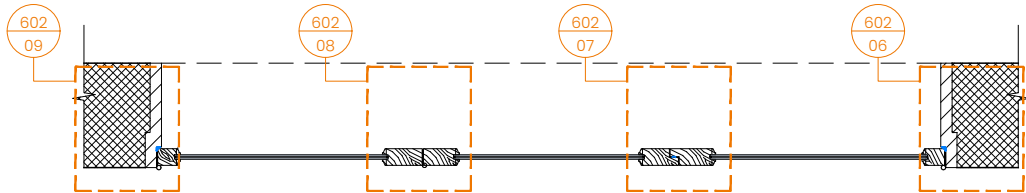
[ 10 ] DT02 DOOR - PLAN DETAIL
