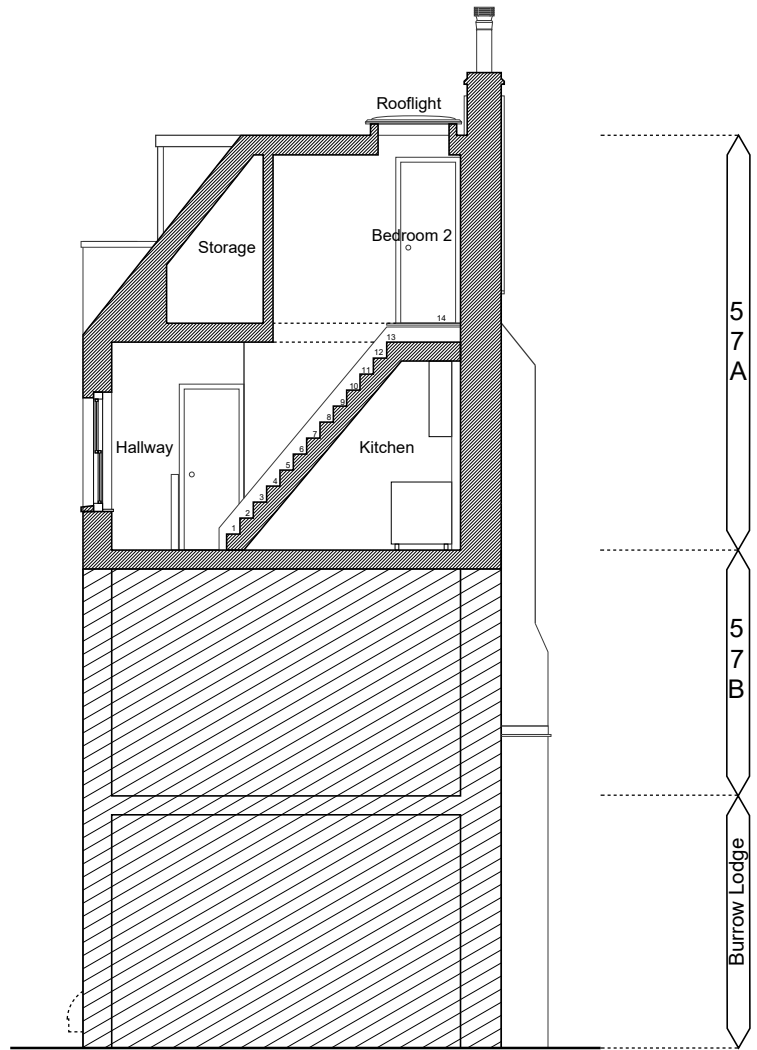
Existing Section BB'
