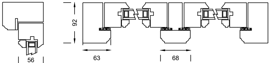
Proposed Glazing & Frame Design
