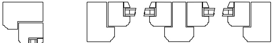
Existing Glazing & Frame Design
