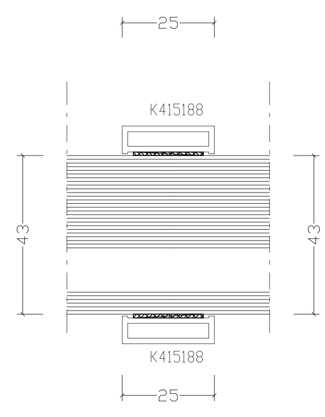
Detail 05 - Transome Detail 1:1@A1
