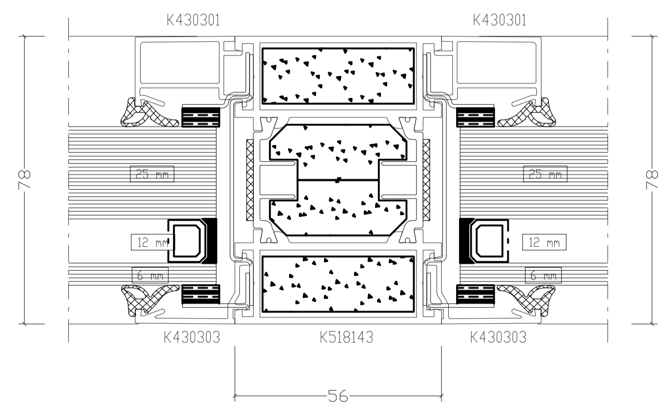
Detail 06 - Transome Detail 1:1@A1
