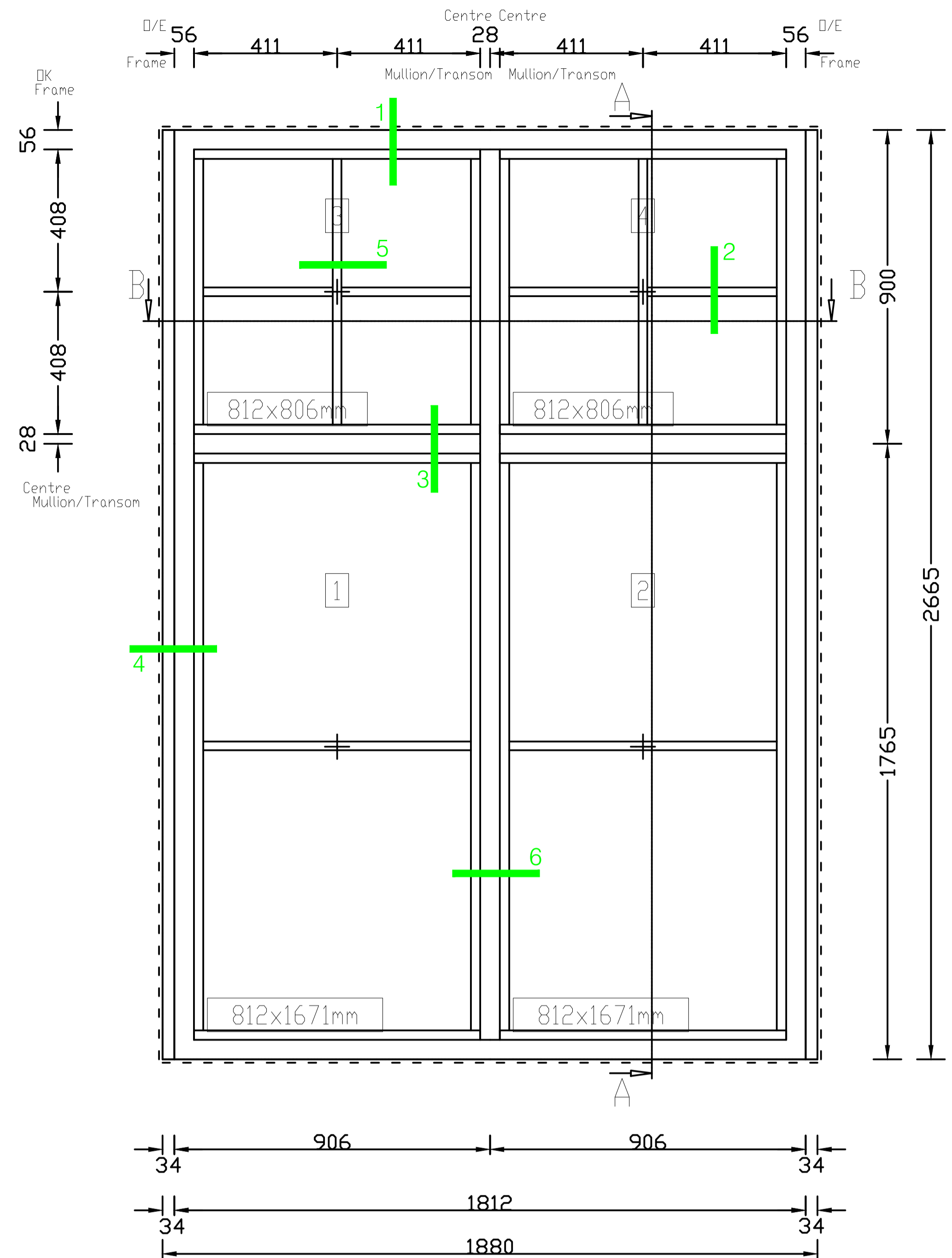
WB.01 - Window Elevation (Exterior View) 1:10@A1
