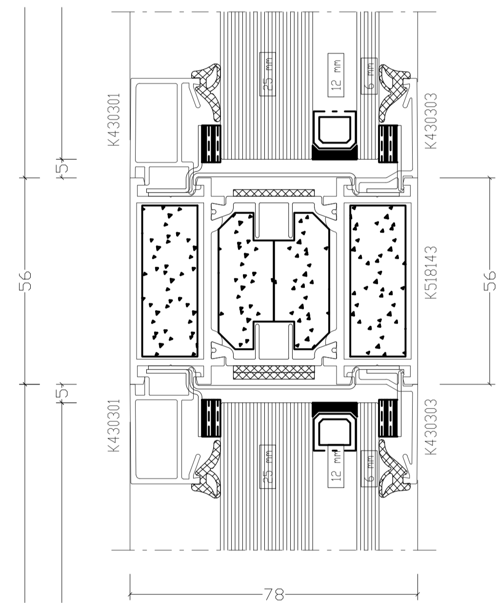
Detail 03 - Transome Detail 1:1@A1
