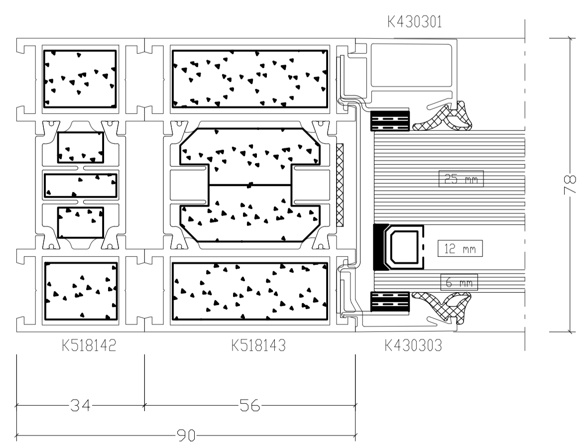
Detail 04 - Reveal Detail 1:1@A1
