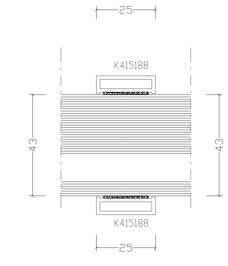
Detail 05 - Transome Detail 1:1@A1
