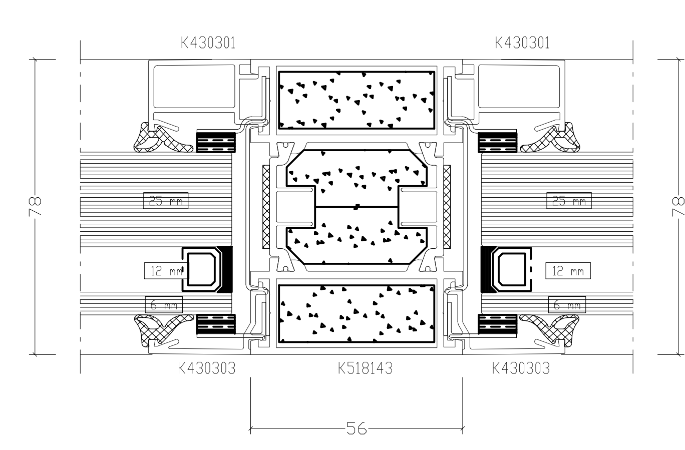
Detail 06 - Transome Detail 1:1@A1
