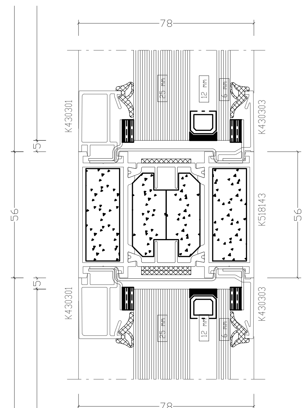
Detail 03 - Transome Detail 1:1@A1
