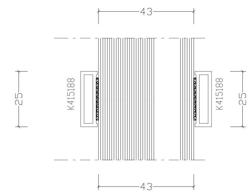
Detail 02 - Transome Detail 1:1@A1
