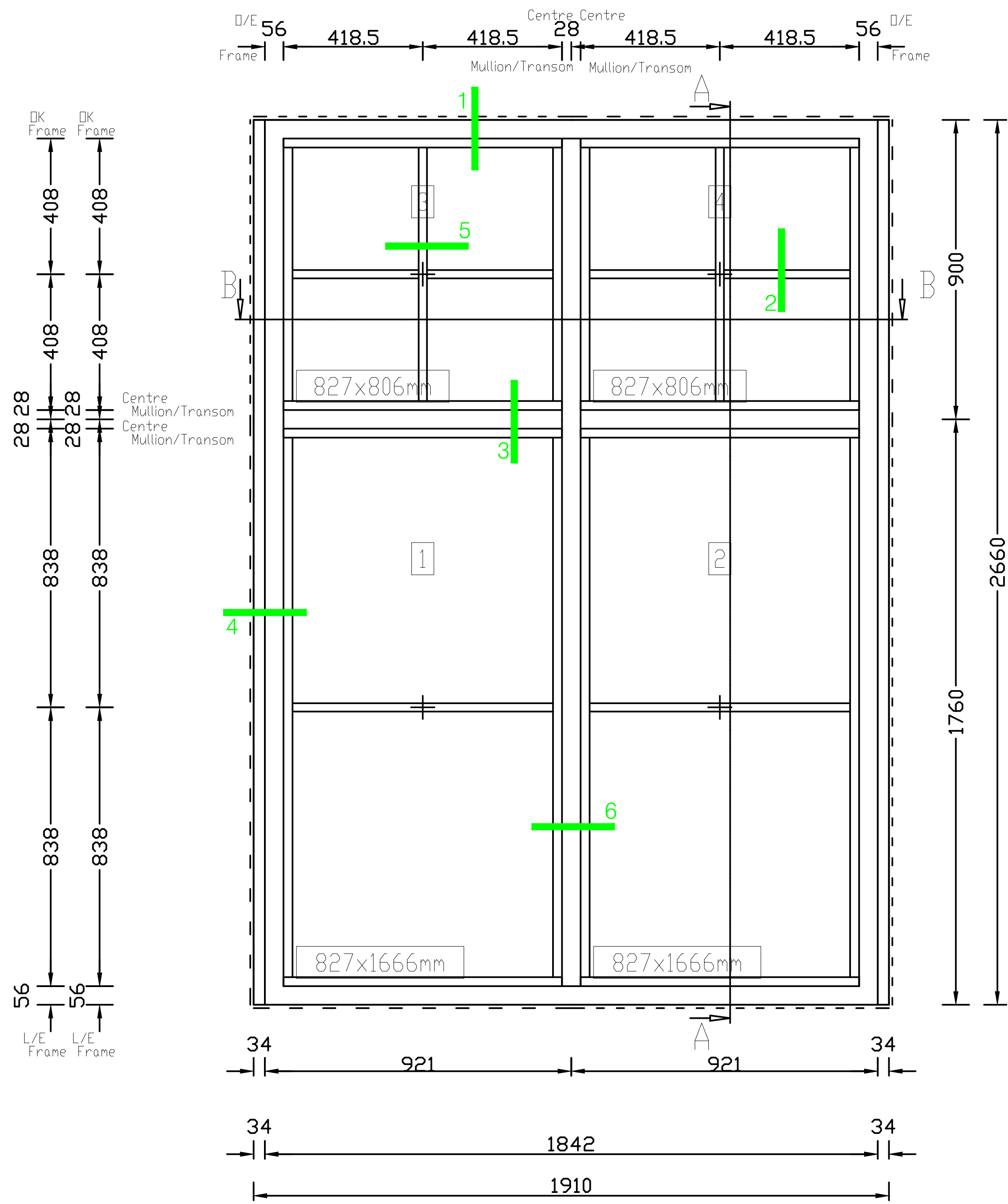
W0.02 - Window Elevation (Exterior View) 1:10@A1
