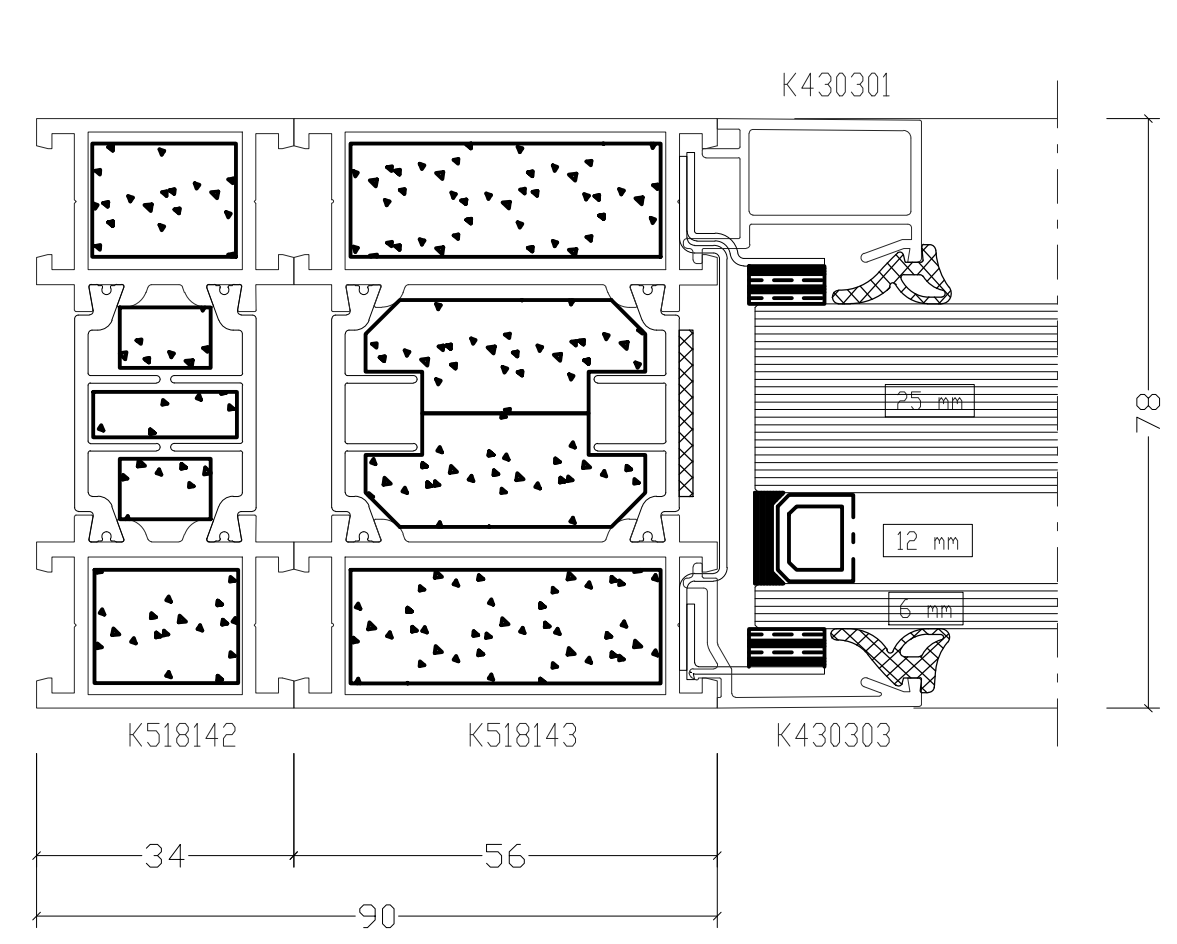
Detail 04 - Reveal Detail 1:1@A1
