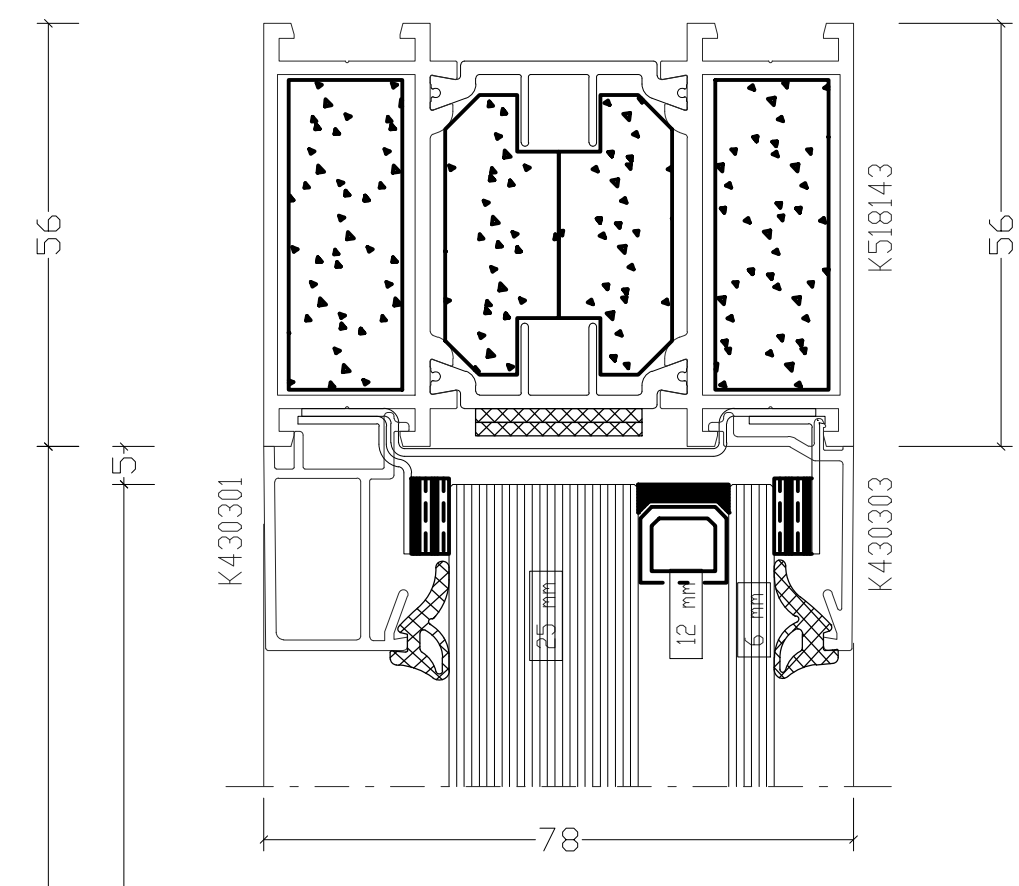
Detail 01 - Head Detail 1:1@A1
