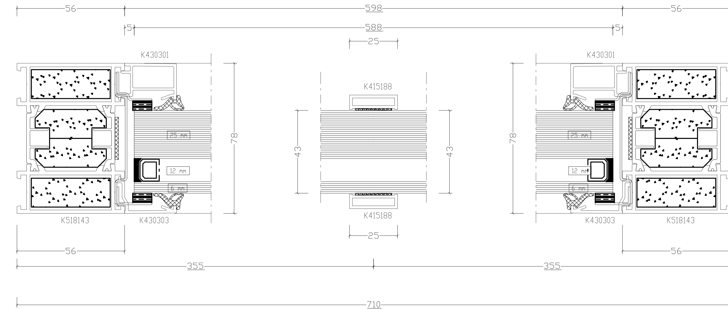
Detail 05 - Reveal Detail 1:1@A1
