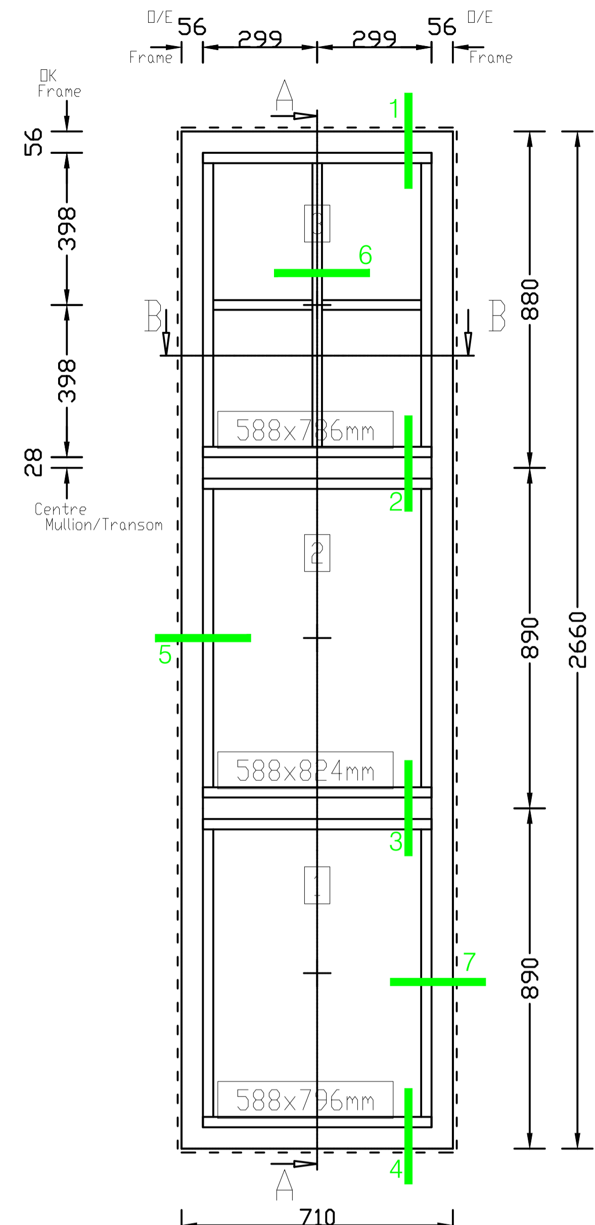
W0.01 - Window Elevation (Exterior View) 1:10@A1
