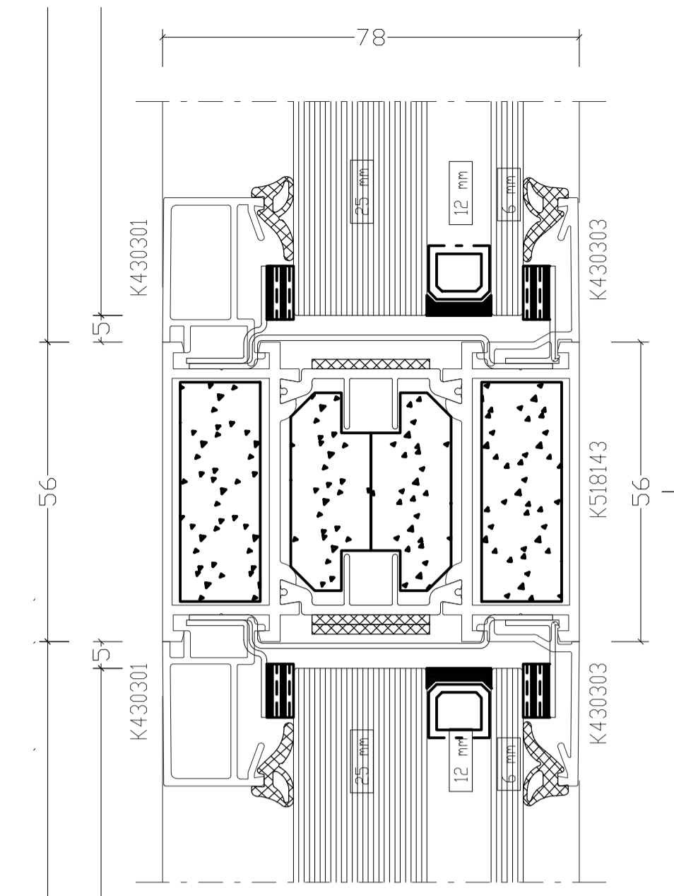
Detail 03 - Transome Detail 1:1@A1
