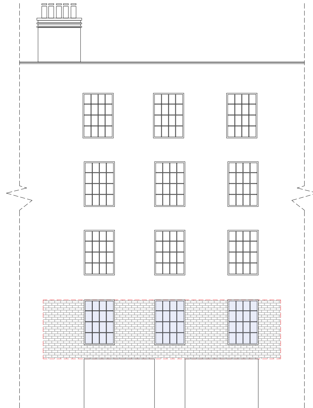
Existing And Proposed East Elevation ( No Proposed Change )
