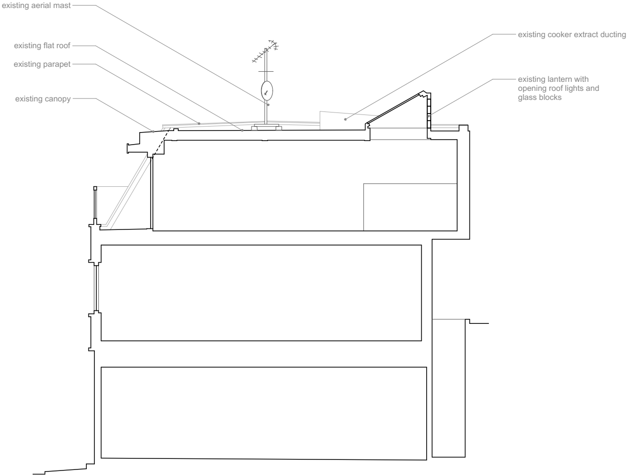
AA Front to Back Section
