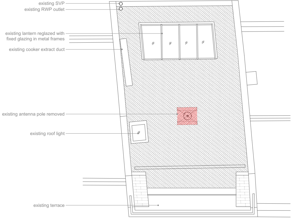
RP Roof Plan
