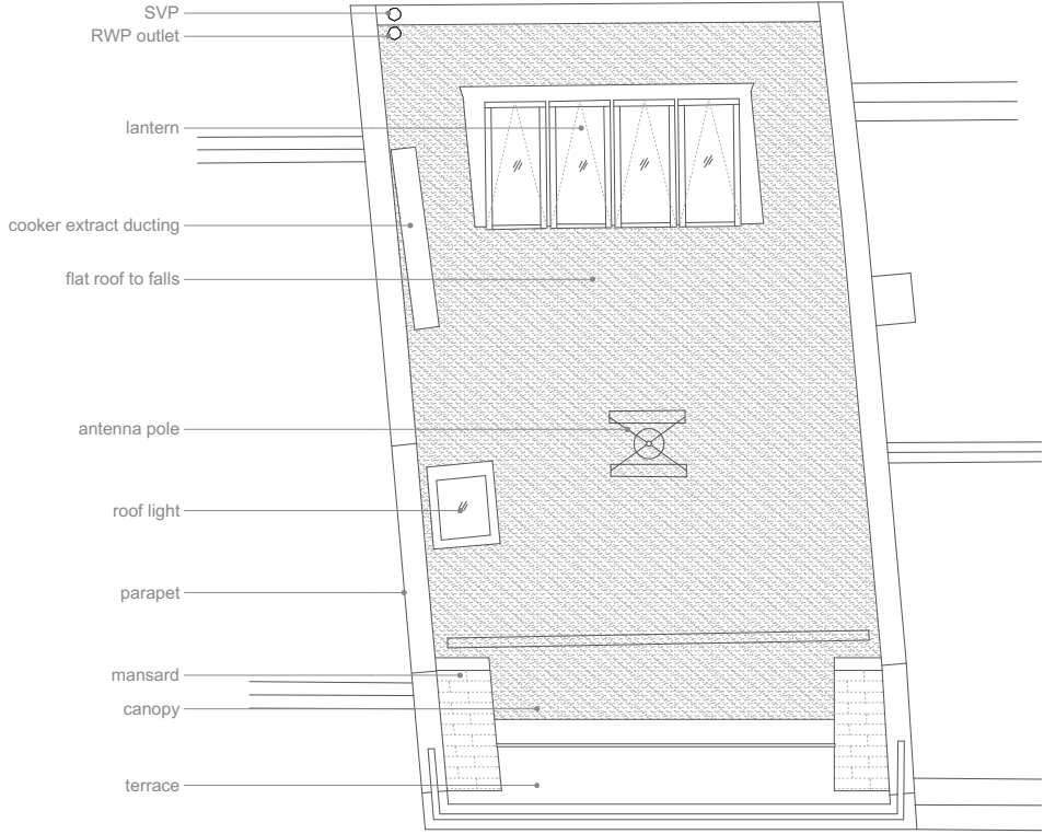
RP Roof Plan
