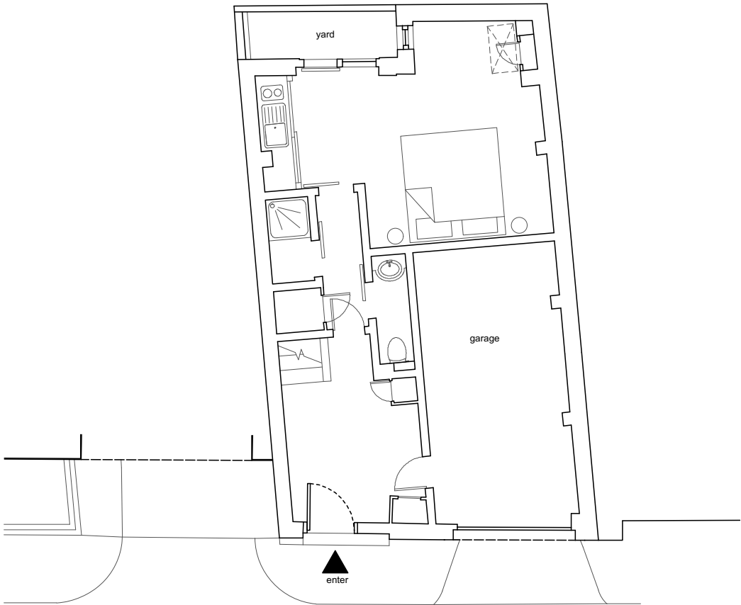
GF Ground Floor Plan
