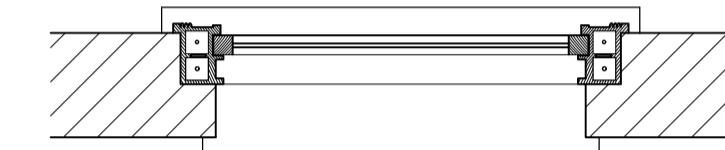
Typical existing timber window Plan
