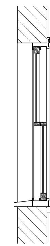
Typical existing timber window section
