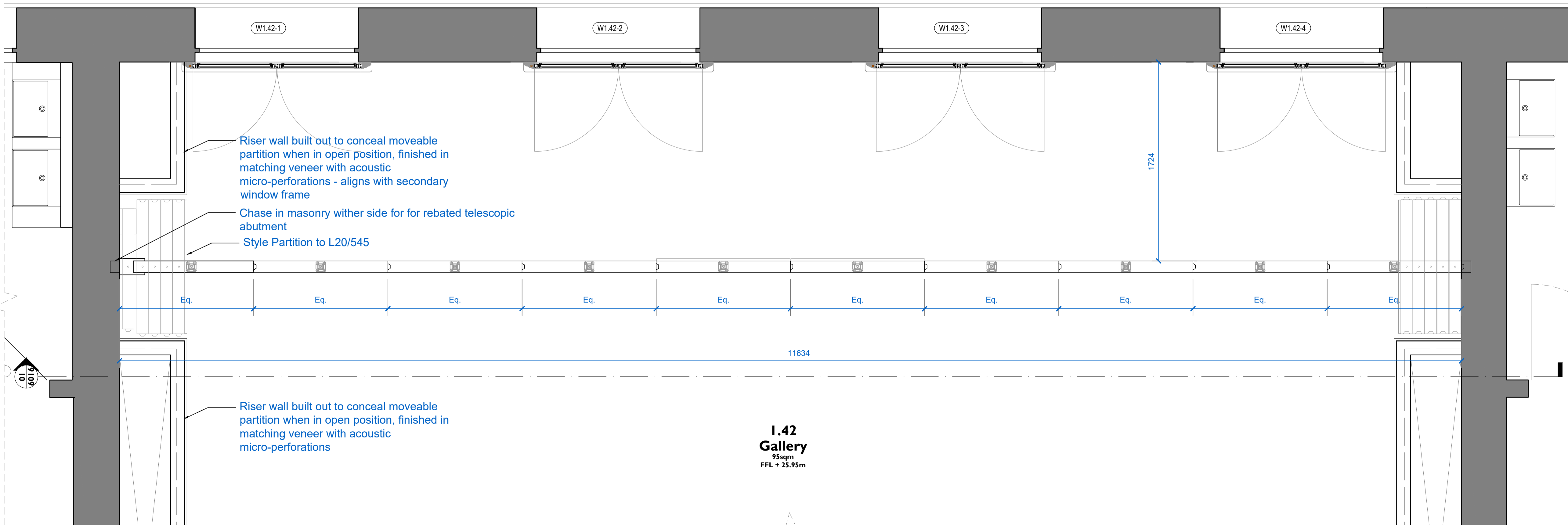
2 L01 GALLERY FOLDING PARTITION PLAN 6004 1:20
