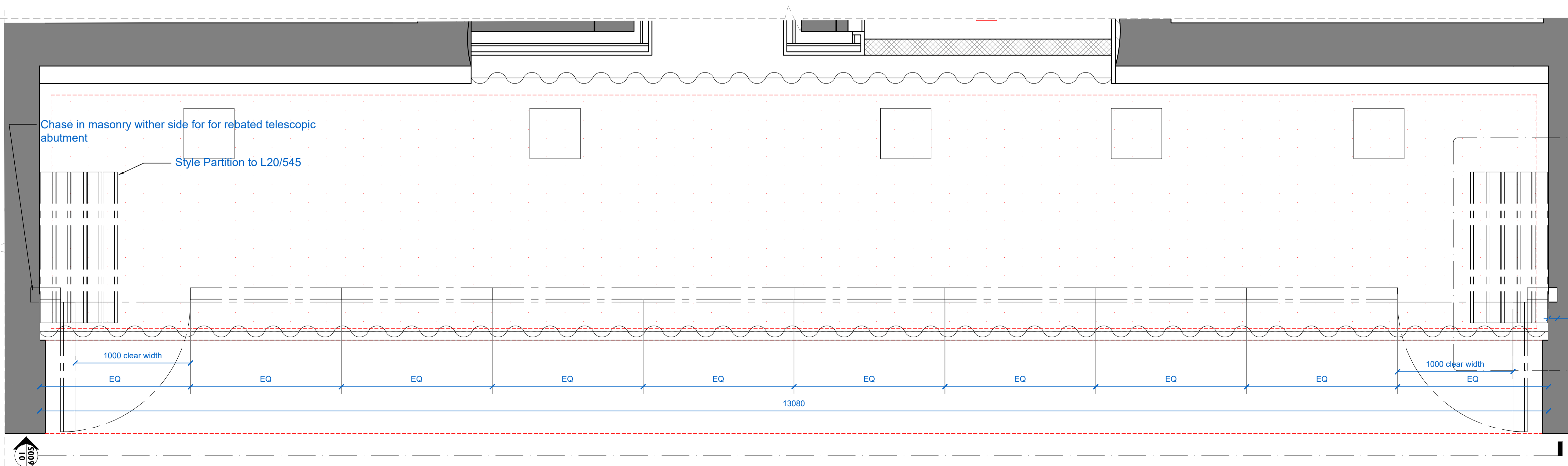
2 EVENT SPACE FOLDING PARTITION PLAN 6005 1:20
