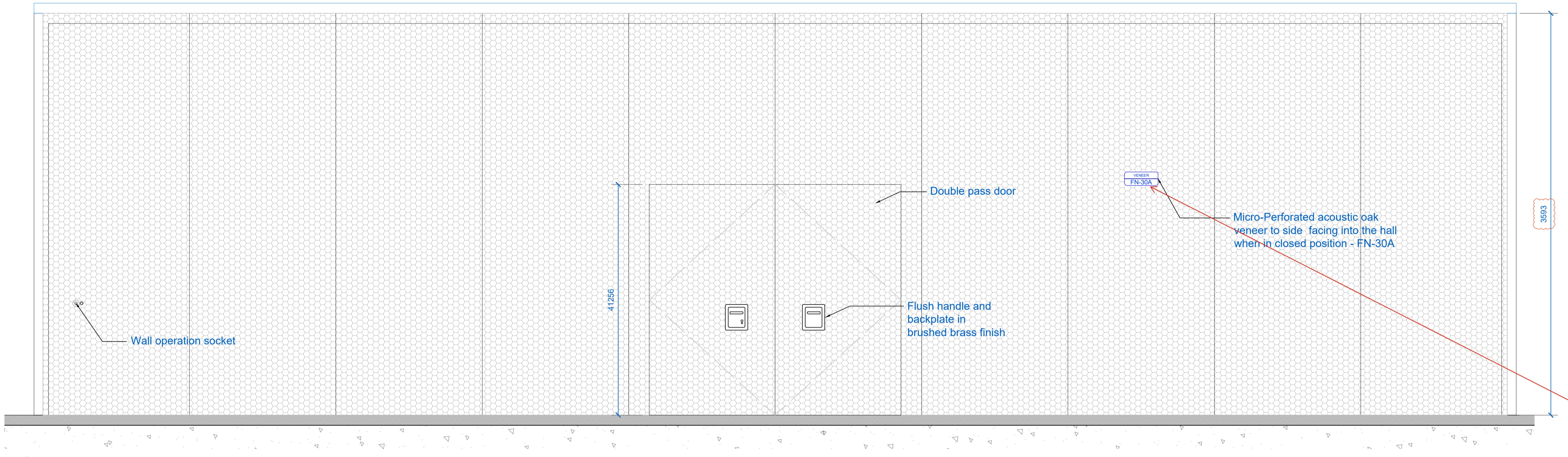
1 TW ENTRANCE FOLDING PARTITION ELEVATION 6004 1:20
